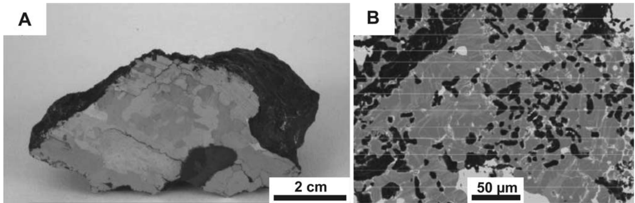
Fig. 1. Silicate nodule in Morasko IAB-MG octahedrite. A. Kamacite and taenite matrix with dark-grey nodule. B. BSE image of alkali feldspar with troilite (white) and graphite (black) in the nodule.
