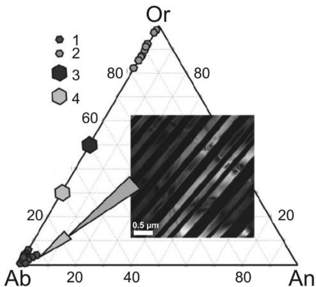
Fig. 4. Feldspar composition (EMPA data) and microtexture. Inset image – TEM dark-field image of periodic twinning in an albite lamella in the intergrown phases (scale bar: 0.5 μm). Abbreviations: 1 – K-rich lamella in the intergrown phases, 2 – Na-rich lamella in the intergrown phases, 3 and 4 – feldspar compositions prior to coarsening (see text for explanations). The composition marked as “3” seems the most likely.
