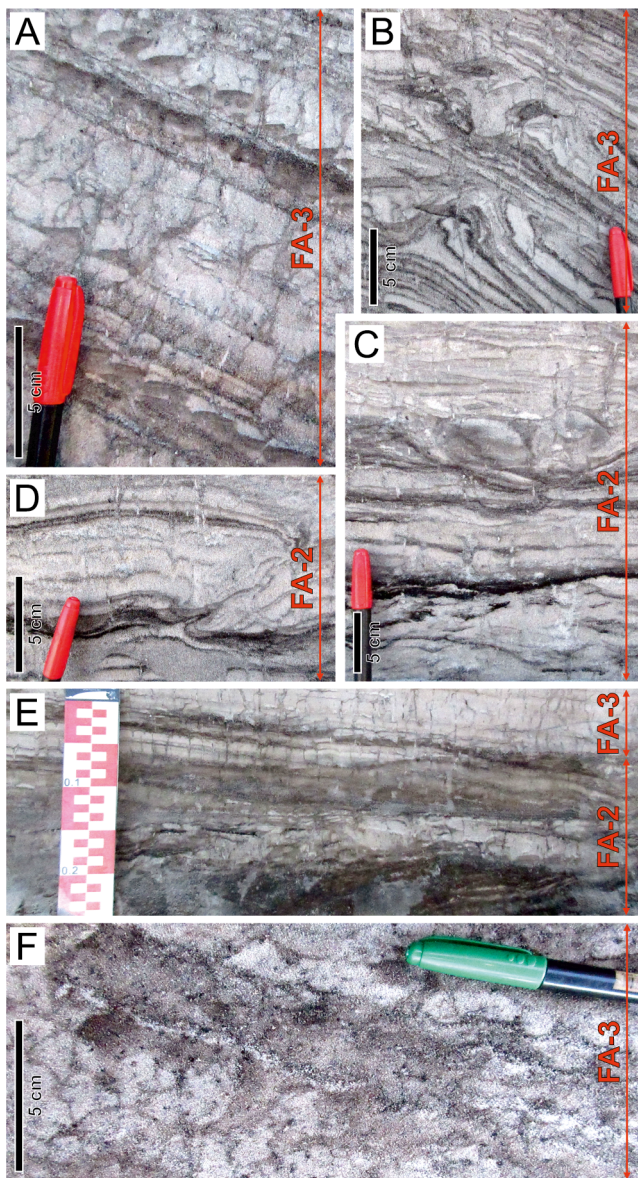
Fig. 8. Brittle and ductile deformation structures in the Józwin IIB opencast mine. A, E, F. Example of brittle deformation – tectonic breccia. B–D. Example of ductile deformations – load casts and flame structures (modified from Chomiak et al. , 2019). Note the superposition of brittle deformation over ductile deformation in Figure 8B–D. For explanations, see the text.
