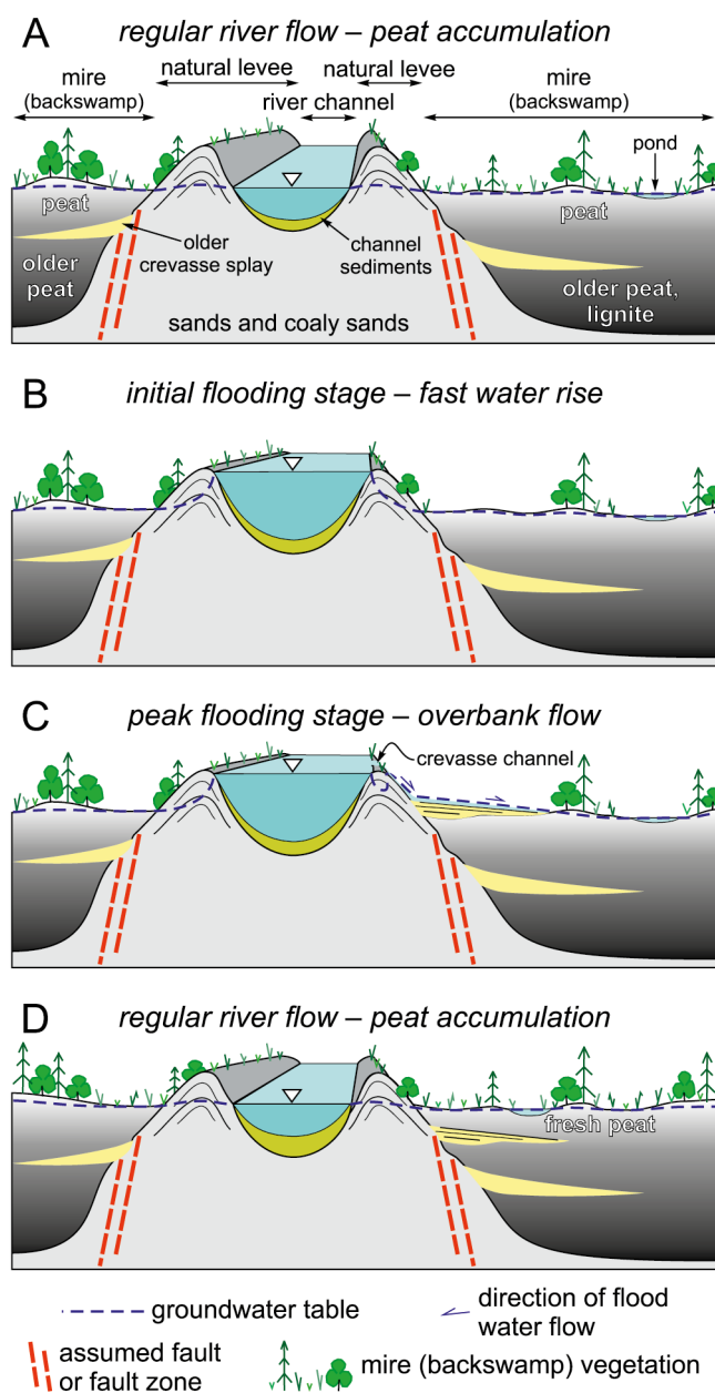
Fig. 14. Conceptual model of subaerial facies formation during a short flood. For explanations, see the text.
