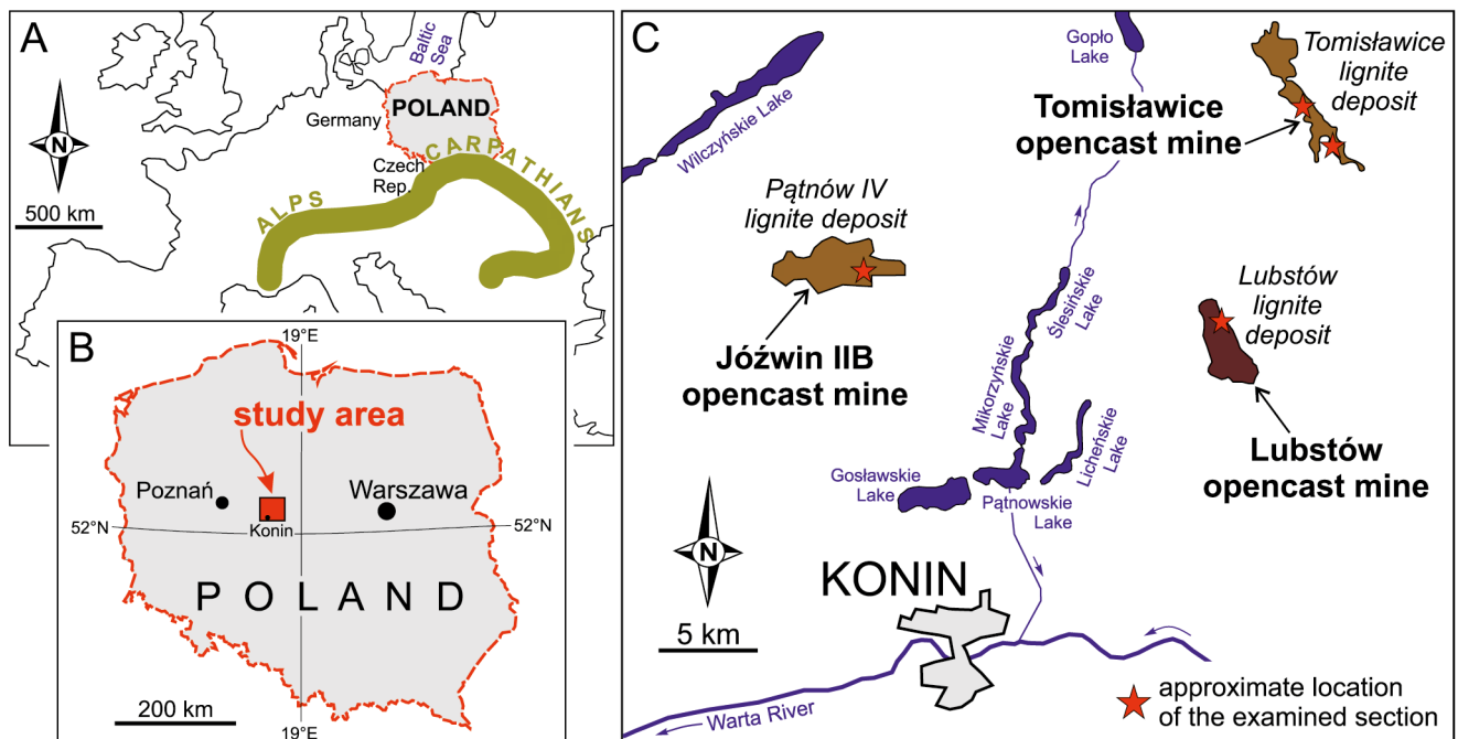
Fig. 1. Location maps. A. Poland on a map of Europe. B. Study area on a map of Poland. C. Location of the examined sections within lignite opencast mines in the Konin Basin. Geographical coordinates of the sections: Lubstów – 52°22′54.8″N, 18°27′46.4″E; Józwin IIB – 52°24′13.2″N, 18°10′56.7″E; Tomisławice South – 52°27′06.3″N, 18°31′46.3″E; Tomisławice North – 52°28′20.7″N, 18°30′38.7″E.
