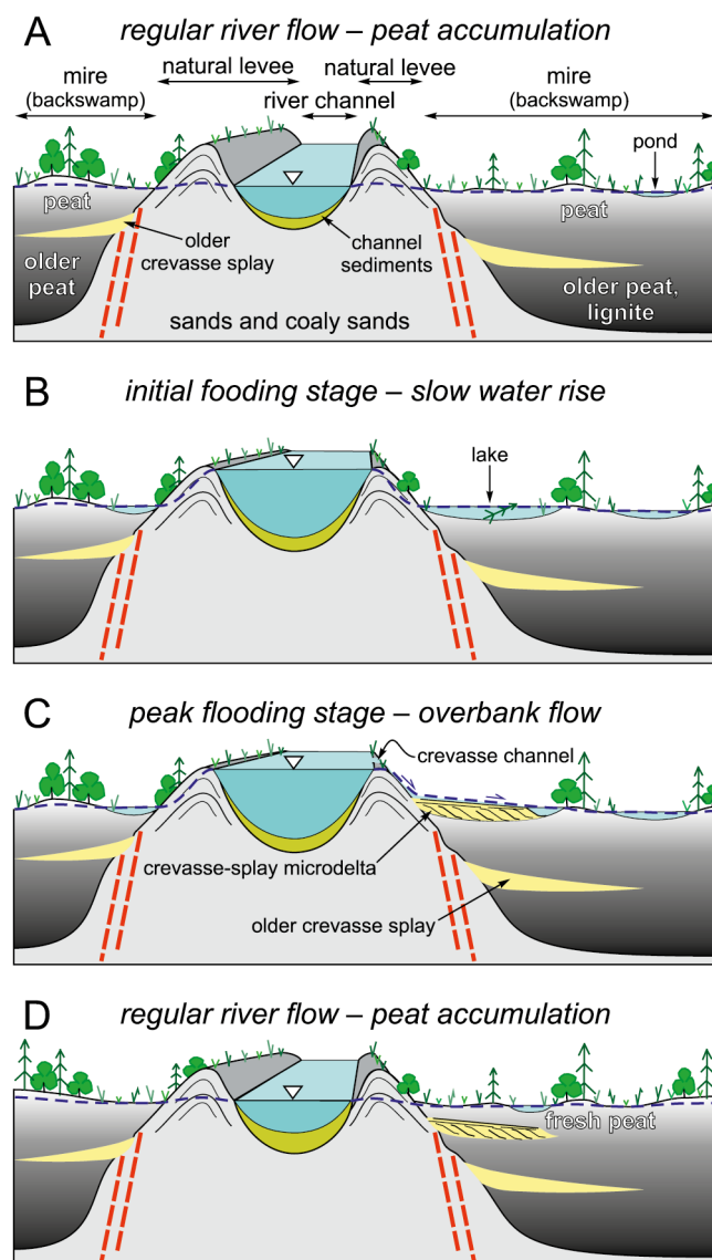
Fig. 15. Conceptual model of subaqueous facies formation during a long, regular flood. For explanations, see the text.
