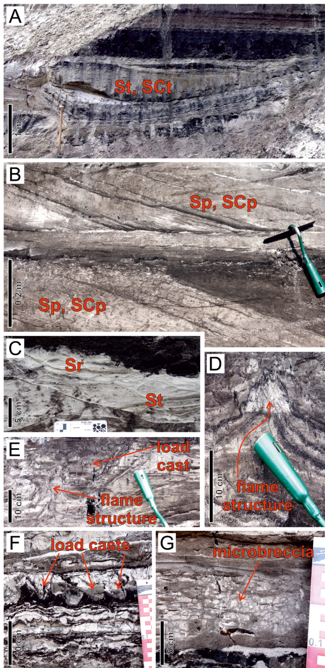
Fig. 12. Non-deformational and deformational structures in the Tomisławice opencast mine, northern site. A–C. Large- and small-scale cross-stratification. D–G. Ductile (load casts and flame structures) and brittle (tectonic microbreccia) structures. For explanations, see Table 1 and the text.
