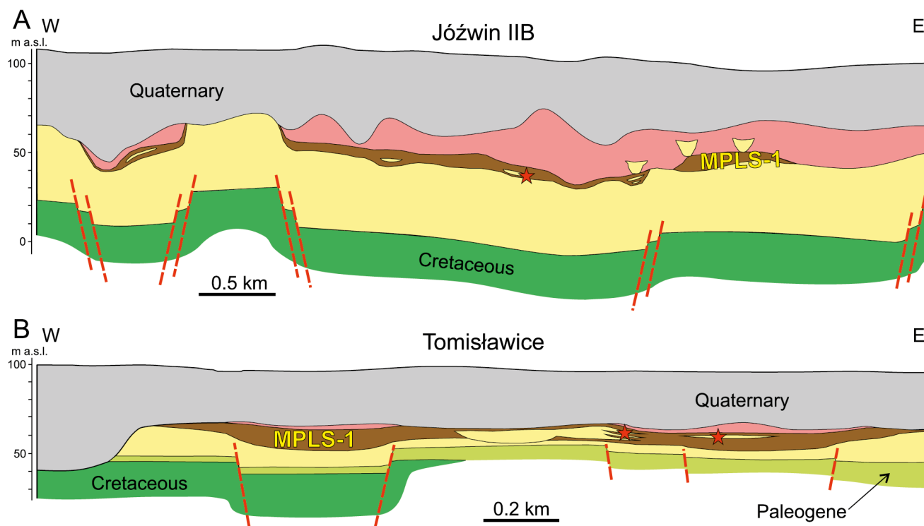
Fig. 4. Geological cross-sections through the Józwin IIB and Tomisławice lignite deposits (modified from Chomiak et al. , 2019; Widera et al. , 2026). Note the approximate stratigraphic position of the examined sediments within the 1st Mid-Polish Lignite Seam (MPLS-1). For explanations, see Figure 3.
