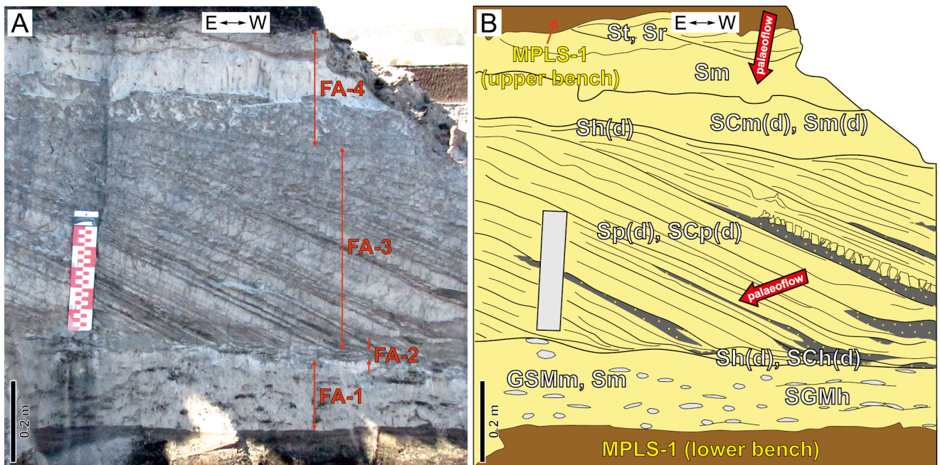
Fig. 7. Interlignite sediments in the Józwin IIB opencast mine. A. Photographic view of the outcrop section (modified from Chomiak et al. , 2019). B. The corresponding line-drawing of the siliciclastic sediments, shown in Figure 7A. For facies codes explanations, as well as descriptions and interpretations of the facies associations, see Tables 1 and 2.
