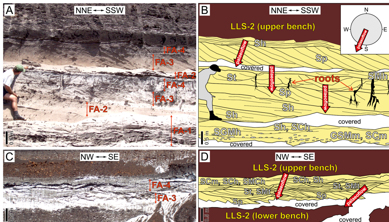
Fig. 5. Interlignite sediments in the Lubstów opencast mine. A, C. Photographic view of the outcrop sections. B, D. The corresponding line-drawings of the siliciclastic sediments, shown in Figure 5A, C, respectively. Note the key (top-right corner), explaining the averaged palaeoflow directions; for facies codes explanations, as well as descriptions and interpretations of the facies associations, see Tables 1 and 2.
