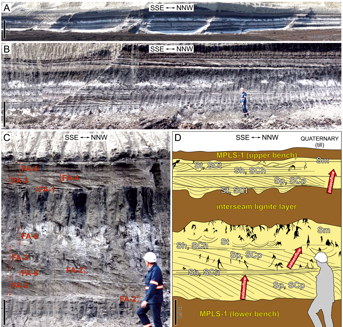
Fig. 11. Interlignite sediments in the Tomisławice opencast mine, northern site. A, B. Panoramic views of the outcrop sections. C. Close-up view of the outcrop section, displaying main facies associations: FA-1-FA-3, and FA-6. D. The corresponding line-drawing of the sediments shown in Figure 11C. Note the repeated occurrence of facies sets in the section. For facies codes explanations, as well as descriptions and interpretations of the facies associations, see Tables 1 and 2.
