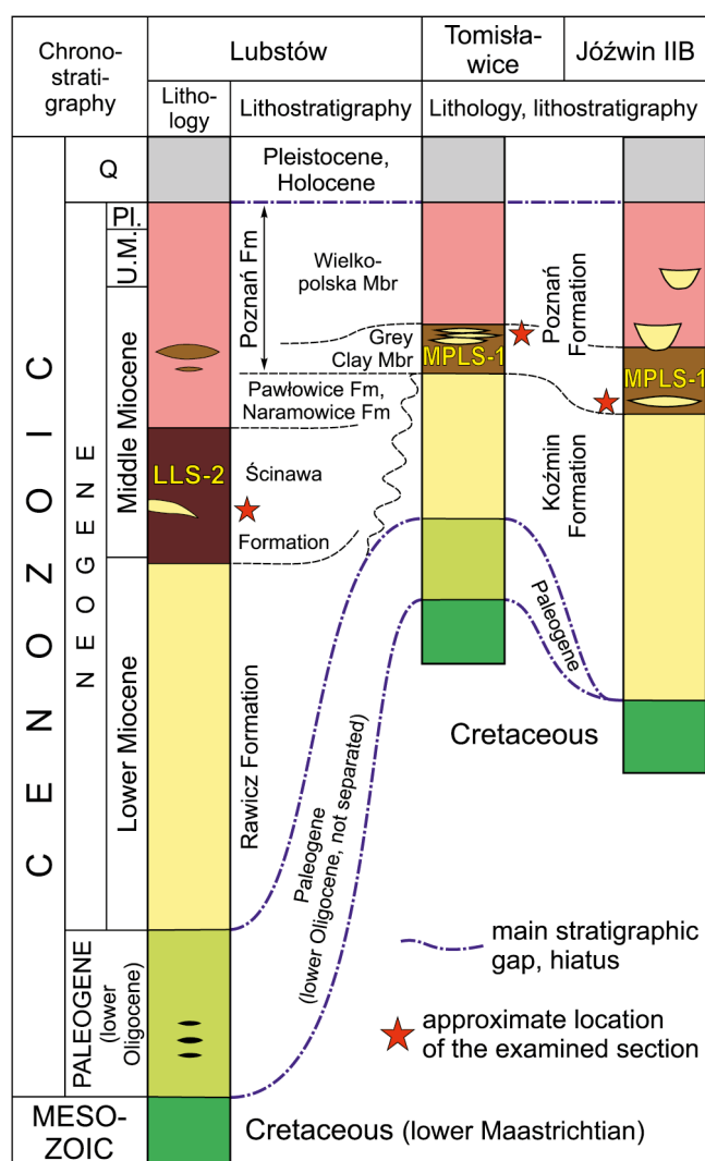
Fig. 2. Generalised lithostratigraphy of areas with mined lignite seams in the Konin Basin. Note the approximate stratigraphic position of the examined siliciclastic sediments within the lignite seams; for explanations, see Figure 3.
