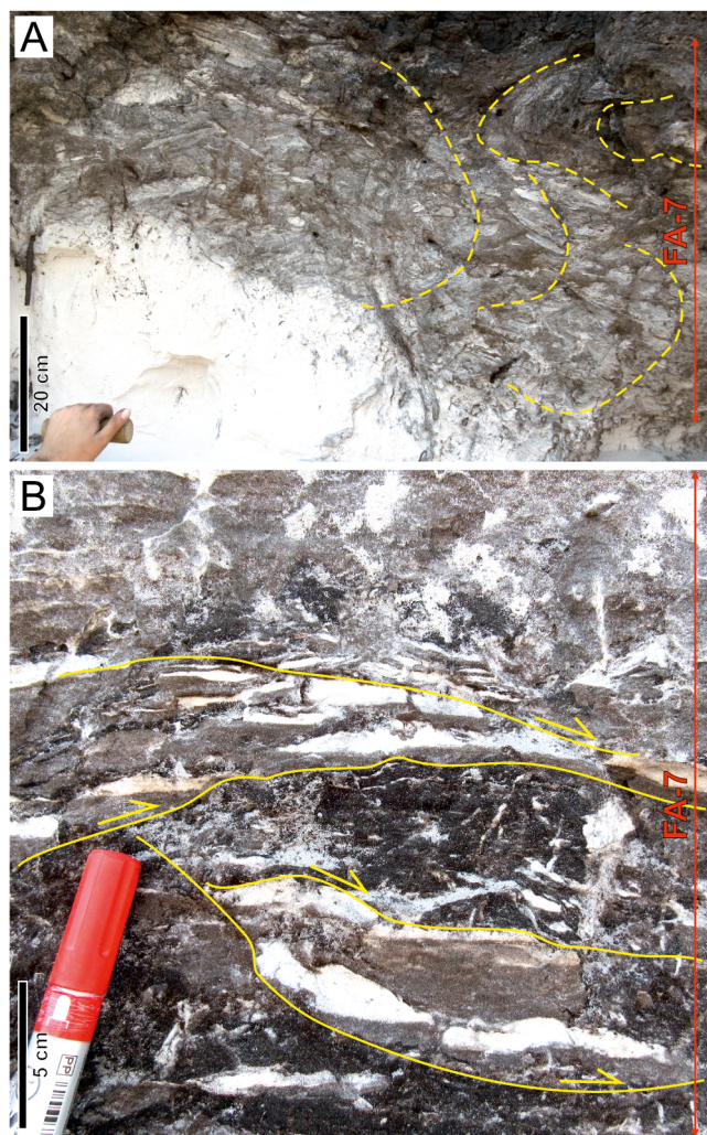
Fig. 10. Sedimentary breccia in the Tomisławice opencast mine, southern site. A. Example of folding (slumping). B. Example of faulting. For explanations, see the text.
