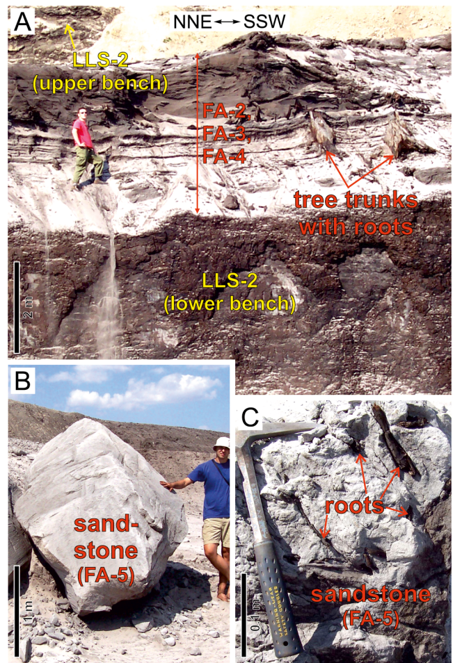
Fig. 6. Special elements and (litho)facies, associated with interlignite sediments in the Lubstów opencast mine. A. Tree trunks with root systems (stumps) in an upright position. B. Blocks of quartzite sandstones, stored in the internal dump. C. Details of quartzite sandstone with visible fossilised plant roots. For explanations, see the text.
