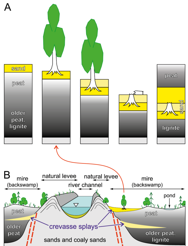
Fig. 13. Fossilisation of tree trunks in an upright position in crevasse-splay sediments (modified after Brzyski et al. , 1976; Gradziński and Doktor, 1995). A. Stages of tree trunks burial as a result of the depositional surface subsidence of the crevasse splay, caused by compaction of the underlying peat/lignite. B. Location of the tree growing on the top of the crevasse splay in relation to the main river channel of the adjacent mire/backswamp. For explanations, see Figure 14 and the text.
