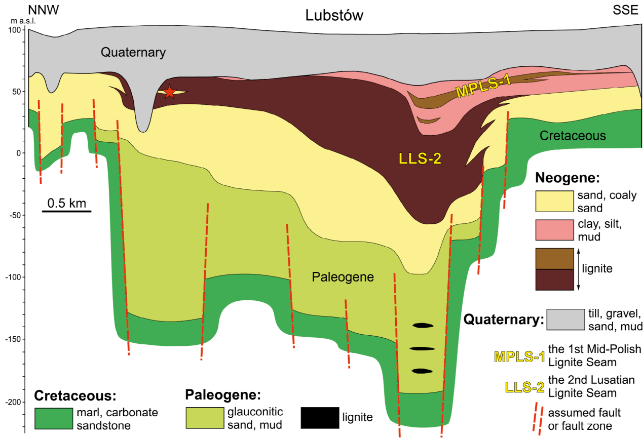
Fig. 3. Geological cross-section through the Lubstów lignite deposits (modified from Widera, 2021). Note the approximate stratigraphic position of the examined sediments within the 2 nd Lusatian Lignite Seam (LLS-2).
