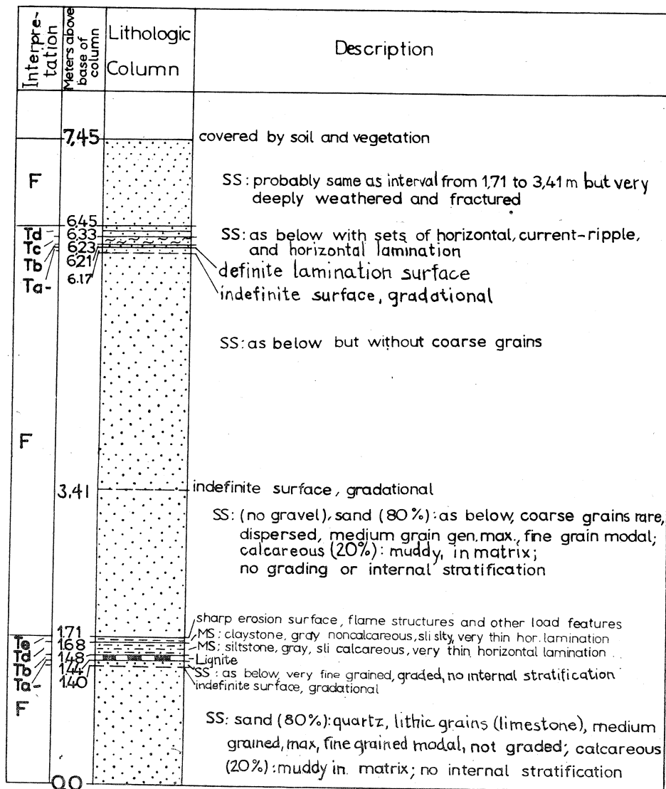
Fig. 11a. Columnar section at Polana (Loc. 6) of Krosno Beds (Lower Oligocene). In lower fluxoturbidite bed (0.00 to 1.71 m), the Ta- interval is thin (1.40 to 1.44 m), and the Tb interval appears to be represented by lignite (1.44 to 1.48 m), with the Tc missing. In the overlying fluxoturbidite bed (1.71 to 6.45 m), the Ta- interval is also thin (6.17 to 6.21 m)
