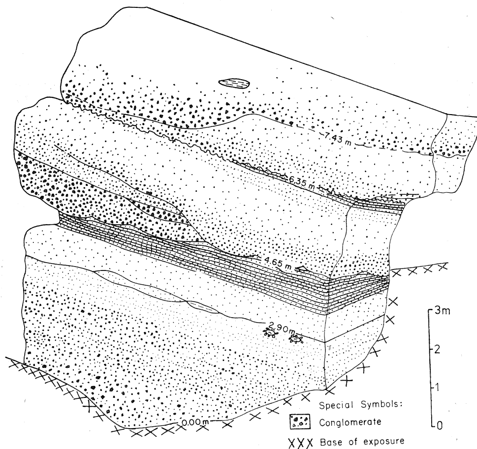
Fig. 8b. Block diagram, view southeast, at Sowa. Fig. 8a is located on right side. Several beds are truncated by erosion surfaces of moderate relief. (Modified from Koszarski, 1956, 1963)
