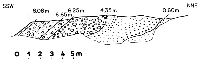
Fig. 7b. Cross section, south—southwest — north — northeast, at Mucharz. Structural dip is 40° south. Bedding surfaces at 0.60, 4.35, 6.25, 6.65, and 8.08 m above base of columnar section are labelled
