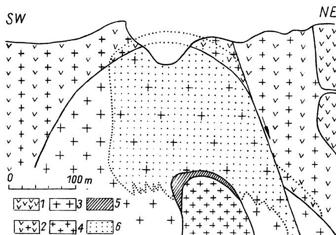
Fig. 2. Geological cross-section illustrating the tin deposit of Altenberg, cited by Schust (1976). 1 - quartz porphyries of Tepliz, 2 - granite porphyries of Altenberg, 3 - exterior granites, 4 - interior granites, 5 - pegmatites, 6 - greisen bodies
