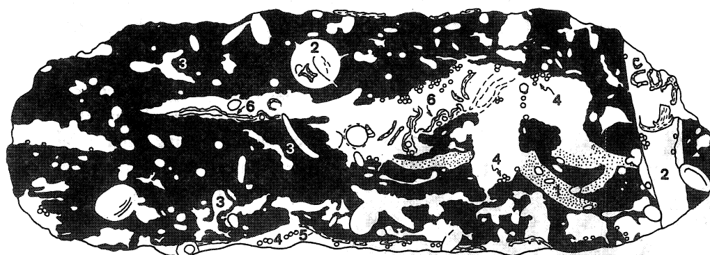
Fig. 6. Vertical section of strongly bored clast (same clast as in Pl. II: 4 and Pl. III). Large cavity in central part of the clast represents probably fragment of Thalassinoides -type burrow. 1 – bioturbations, 2 – bivalve borings, 3 – polychaeta borings, 4 – serpulids, 5 – oysters, 6 – microstromatolite structures (see Pl. III: 3)
