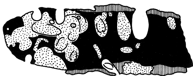
Fig. 4. Strongly bored clast (black) with several generations of bivalve borings and a bio-genic layer (vertical rules) composed of oysters and serpulids (see Pl. VI: 6). Partly abraded borings are filled with various sediments (dotted). Some borings cut across the bio-genic layer
