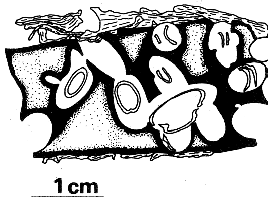
Fig. 5. Vertical section of bored clast showing Fe-stained zone around borings and at clast margin (black and stippled). Some borings with shells of resident bivalves and some with bioclasts. Clast is encrusted by oysters and serpulids which are locally bored by bivalve. See Pl. VII: 1
