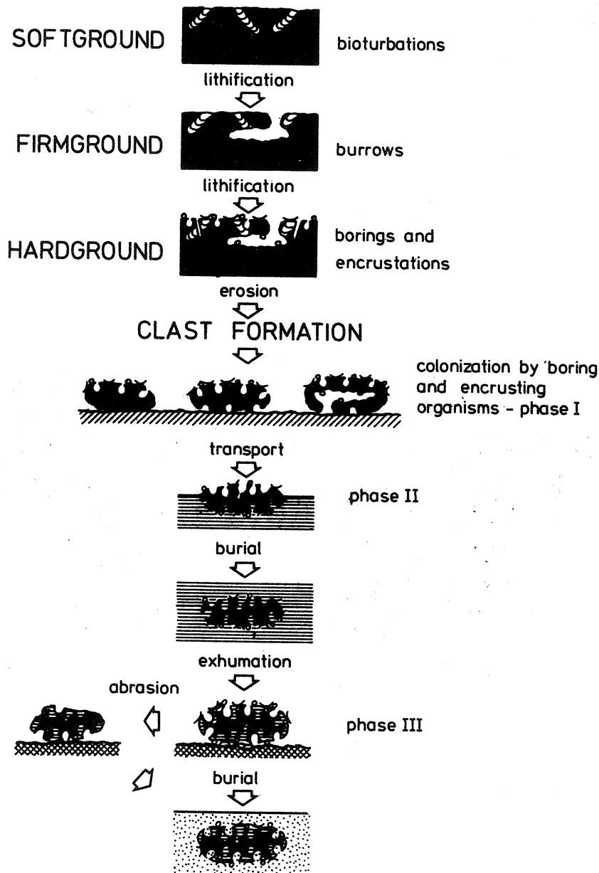
Fig. 10. History of origin of bored and encrusted clasts
