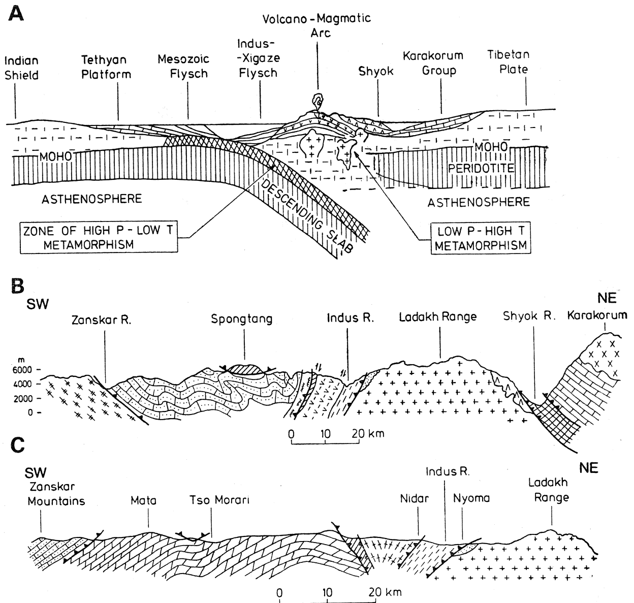
Fig. 4. Cross-sections of the Indus-Tsangpo suture zone. A. Schematic model for the evolution of Indus-Tsangpo suture zone prior to the collision of the Indian and Tibetan plates. B. Generalized geological cross-section through the Central Ladakh. C. Generalized geological cross-section through the South-eastern Ladakh
