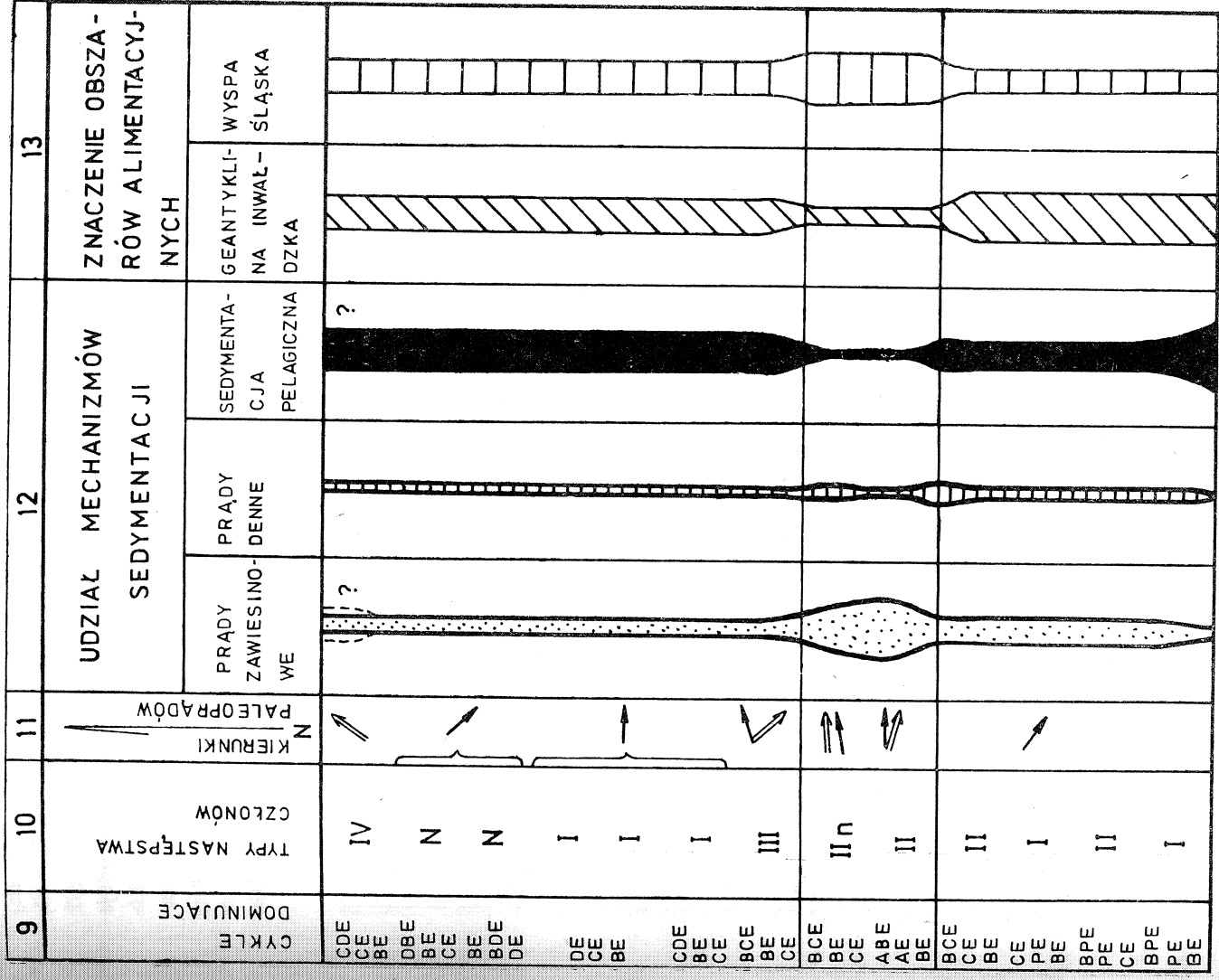
Fig. 19. Main characteristics and sedimentological interpretation of Cieszyn Beds from Żywiec region. For explanation, see caption in Fig. 18
