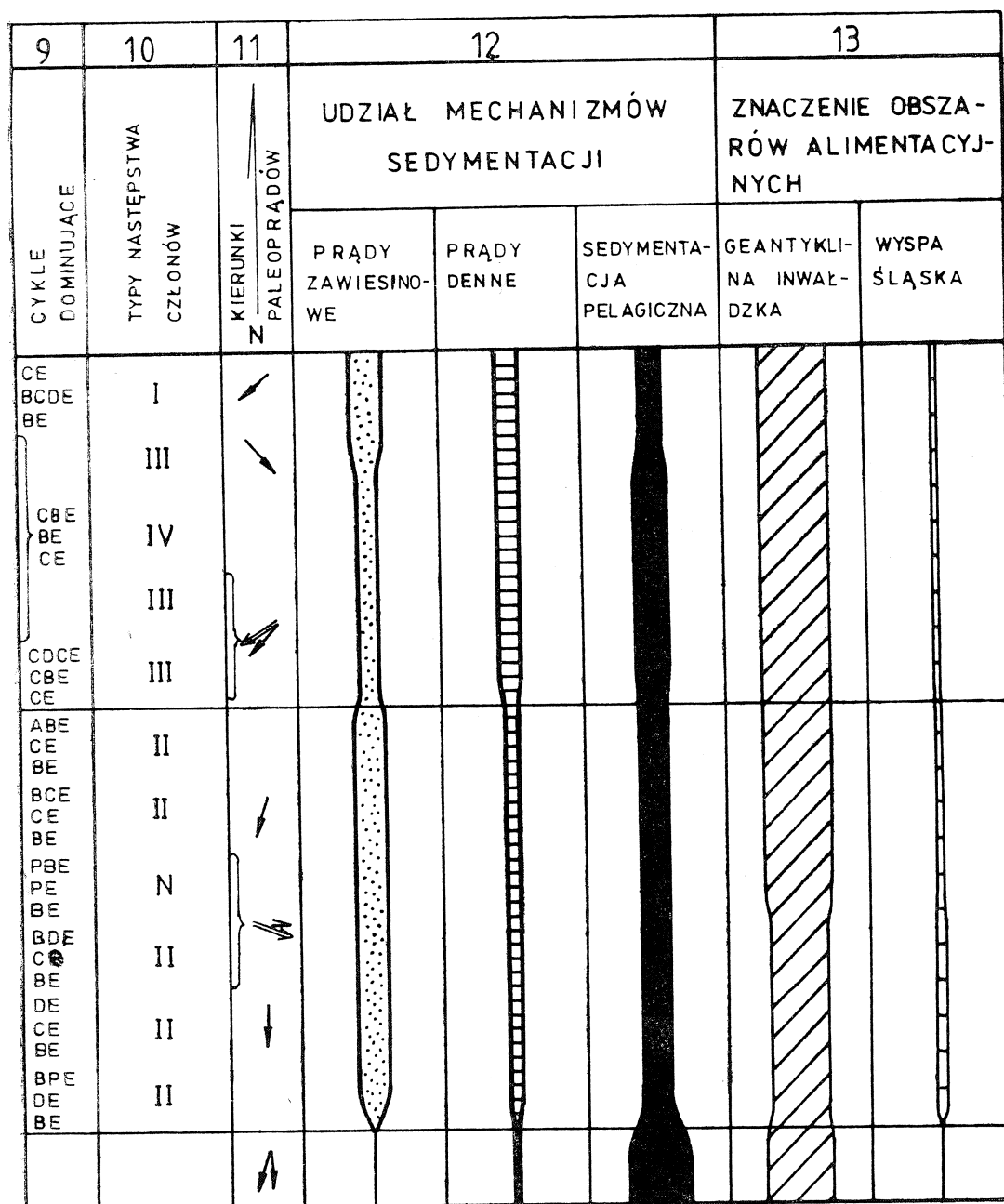
Fig. 20. Main characteristics and sedimentological interpretation of Cieszyn Beds in Bielsko-Biała region. For explanation, see caption in Fig. 18
