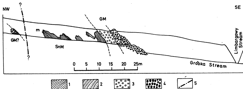
Fig. 5. Exposure of exotic limestone-bearing conglomerates of the Gróbkka Member (Sromowce Formation), Gróbkka Stream, Sromowce (after Birkenmajer & Jednorowska, 1983). 1 — shales, marly shales; 2 — sandstones and siltstones ( m ); 3 — loosely-cemented conglomerate; 4 — hard, well-cemented conglomerate; 5 — faults: GM — Gróbkka Member; SnM — Sneznica Siltstone Member;
