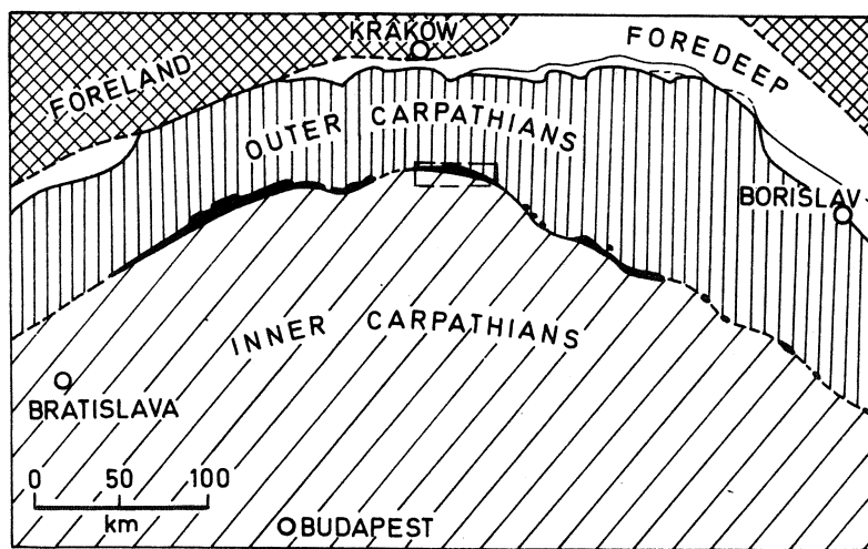
Fig. 1. Key map to show location of the Pieniny Klippen Belt (in black) in the Carpathians. Rectangle — see Fig. 2
