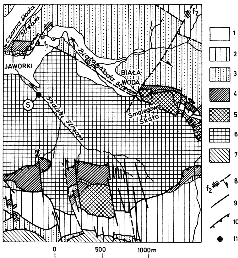
Fig. 6. Geological sketch-map of the Pieniny Klippen Belt, Skalski Stream area, Jaworki (after Birkenmajer, 1979). 1 — Quaternary cover; 2 — Magura Palaeogene flysch (Magura Nappe and Klippen mantle); 3, 4 — Grajcarek Unit (3 — Jarmuta Formation and Malinowa Shale Formation, Upper Cretaceous; 4 — Jurassic and Lower Cretaceous deposits); 5 — Czorsztyn Unit (Jurassic and Cretaceous); 6 — Niedzica Nappe (Jurassic and Cretaceous); 7 — Branisko Nappe (Jurassic and Cretaceous); 8 — Late Tertiary strike-slip faults; 9 — Late Tertiary faults and overthrusts; 10 — Late Cretaceous — Early Tertiary overthrusts; 11 — exotic limestone-bearing site at Skalski Stream (Bukowiny Gravelstone Member, Sromowce Formation)
