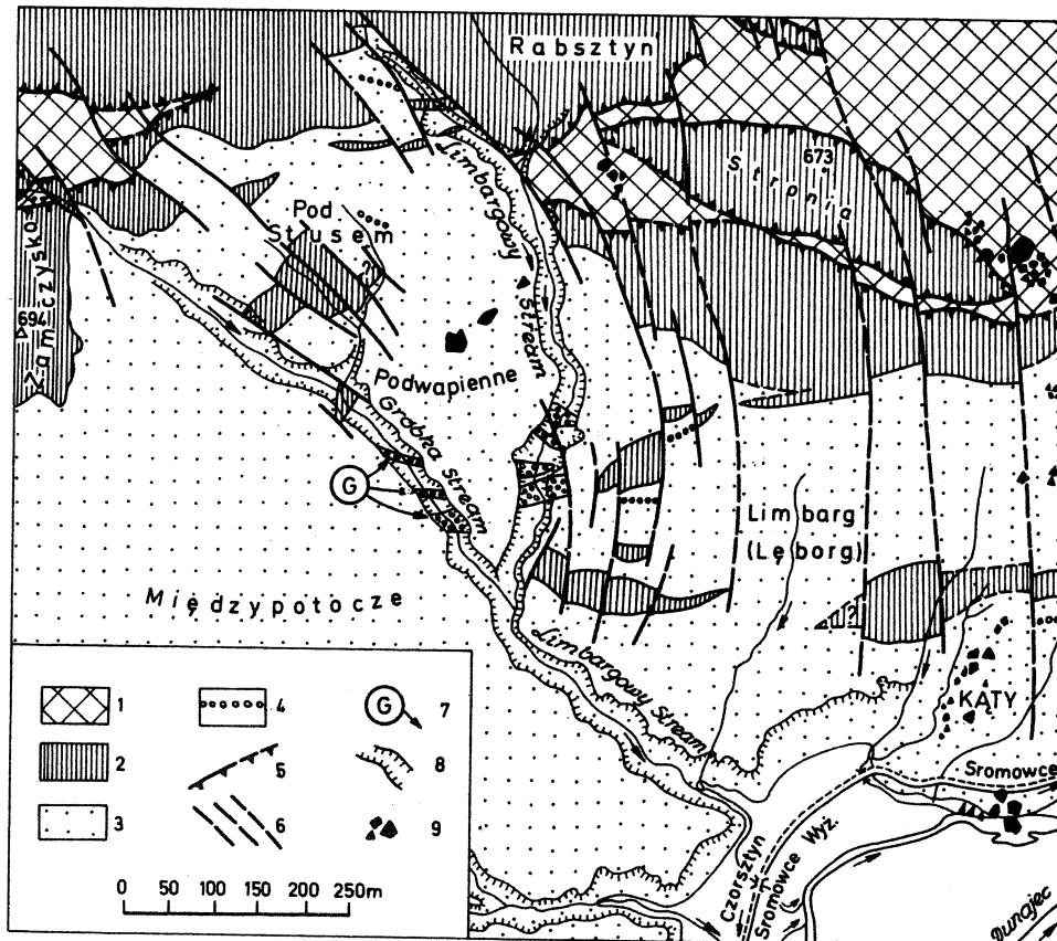
Fig. 4. Position of exotic-bearing conglomerates of the Gróbka Member (Sromowce Formation) in geological map of the Gróbka Stream area, Sromowce (after Birkenmajer & Jednorowska, 1983). 1 — Czorsztyn Unit (Jurassic and Cretaceous); 2, 3 — Branisko Nappe (2 — Jurassic and Neocomian; 3 — Albian-Lower Campanian); 4 — conglomerate intercalations and horizons; 5 — major overthrusts; 6 — faults; 7 — sampling site of exotic limestone pebbles; 8 — escarpments; 9 — large loose limestone blocks from the Czorsztyn Unit
