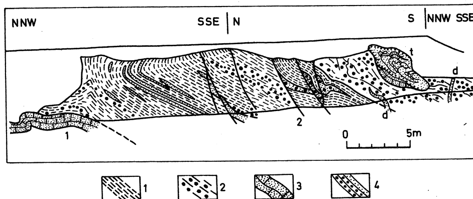
Fig. 7. Exposure of the Bukowiny Gravelstone Member (Sromowce Formation, Niedzica Nappe) at Skalski Stream, Jaworki (after Birkenmajer, 1979). 1 — Sromowce Formation, sandstones; 2 — Bukowiny Gravelstone Member (lithological signatures: 1 — clayshales, clays and marls 2 — gravelly mudstone; 3 — sandstone; 4 — graded sandstone and conglomerate; d — clastic dyke; t — sandstone slump ball)
