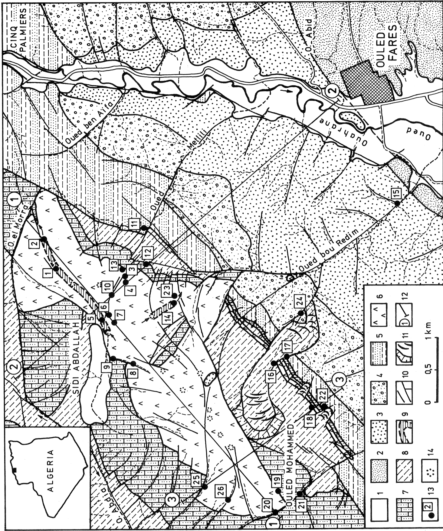
Fig. 1 Geological map of the Ouled Farès area. 1 - recent alluvia, 2 - older Quaternary alluvia, 3 - the oldest Quaternary and Uppermost Pliocene alluvia and other continental sediments, 4 - Upper Pliocene, continental clastic sediments, 5 - Lower Pliocene, continental-marine shallow clastic sediments, 6 - Upper Miocene, Sarmatian (Sahelian), gypsiums, 7 - Upper Miocene, Sarmatian (Sahelian), sandstones, 8 - Upper Miocene, Tortonian, clays, 9 - generalized plan of cave galleries, 10 - linear discontinuities, 11 - landslides, 12 - cross-sections, 13 - sampling sites, 14 - sinkholes
