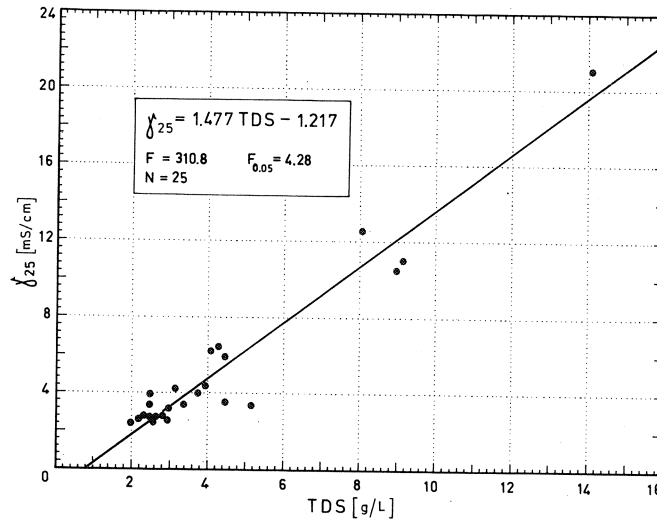
Fig. 4 Conductivity at 25°C ( \gamma_{25} ) versus TDS
