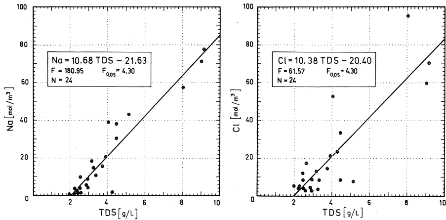
Fig. 6 Concentration of \text{Na}^+ and \text{Cl}^- versus TDS
