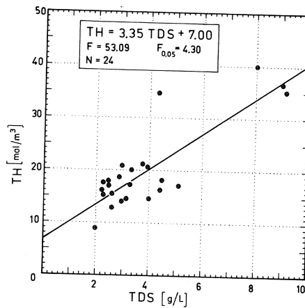
Fig. 9 Total hardness TH versus TDS
