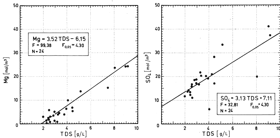
Fig. 7 Concentrations of \text{Mg}^{+2} and \text{SO}_4^{-2} versus TDS
