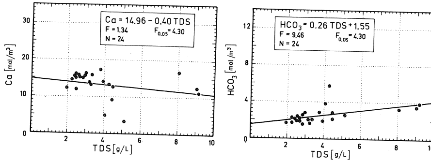
Fig. 8 Concentrations of \text{Ca}^{+2} and \text{HCO}_3^- versus TDS
