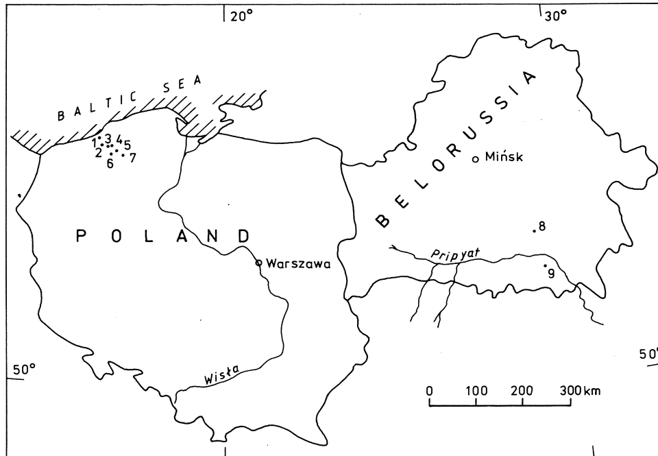
Fig. 1 Map of Poland and Belorussia showing location of boreholes discussed in text. 1 – Sarbinowo 1, 2 – Biesiekierz 1, 3 – Kłanino 1, 4 – Karsina 1, 5 – Drzewiany 1, 6 – Chmielno 1, 7 – Biały Bór 1, 8 – Oktyabrskaya 30, 9 – Zaozemaya 32
