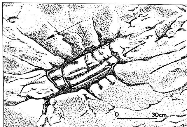
Fig. 3 Break-through prod mark. Upper Cretaceous Flysch. Valea Leurzi, Rumania (after photograph)
