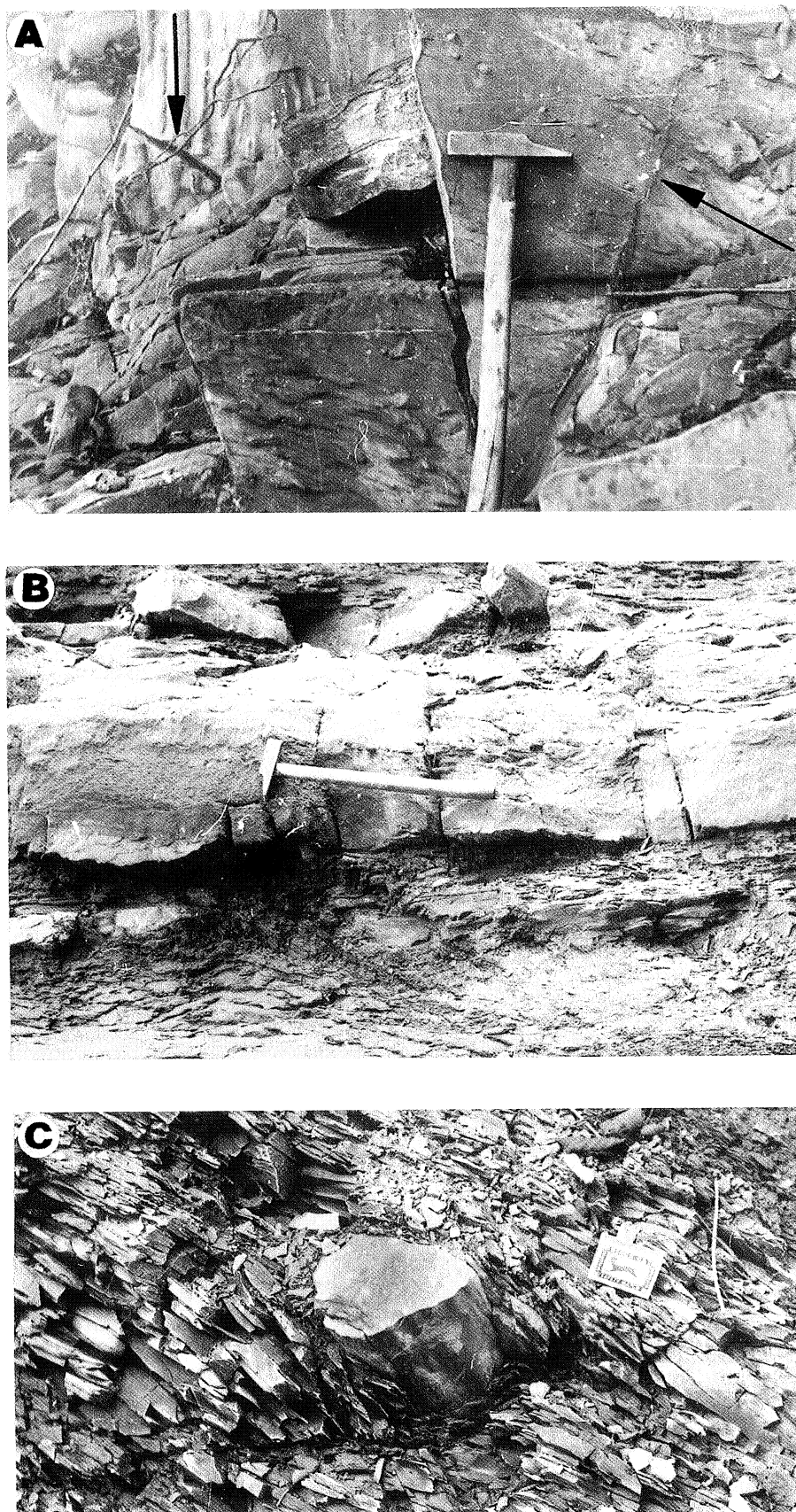
Plate 17 (A) Changing directions of palecurrent markings in succesive flysch beds. Oligocene Krosno Beds, Wernejówka. (B) Amalgamated turbidit bed. Remnants of light coloured lower layer, deposited by current coming from NNW, overlain by coarse grey layer laid down by current coming from SE. Oligocene Krosno Beds, Sieniawa (after Dżułyński & Ślaczka, 1958). (C) Isolated erosion channel (gutter mark) in shales. Direction of flow away from observer. Oligocene Magura Beds, Dragaszów
