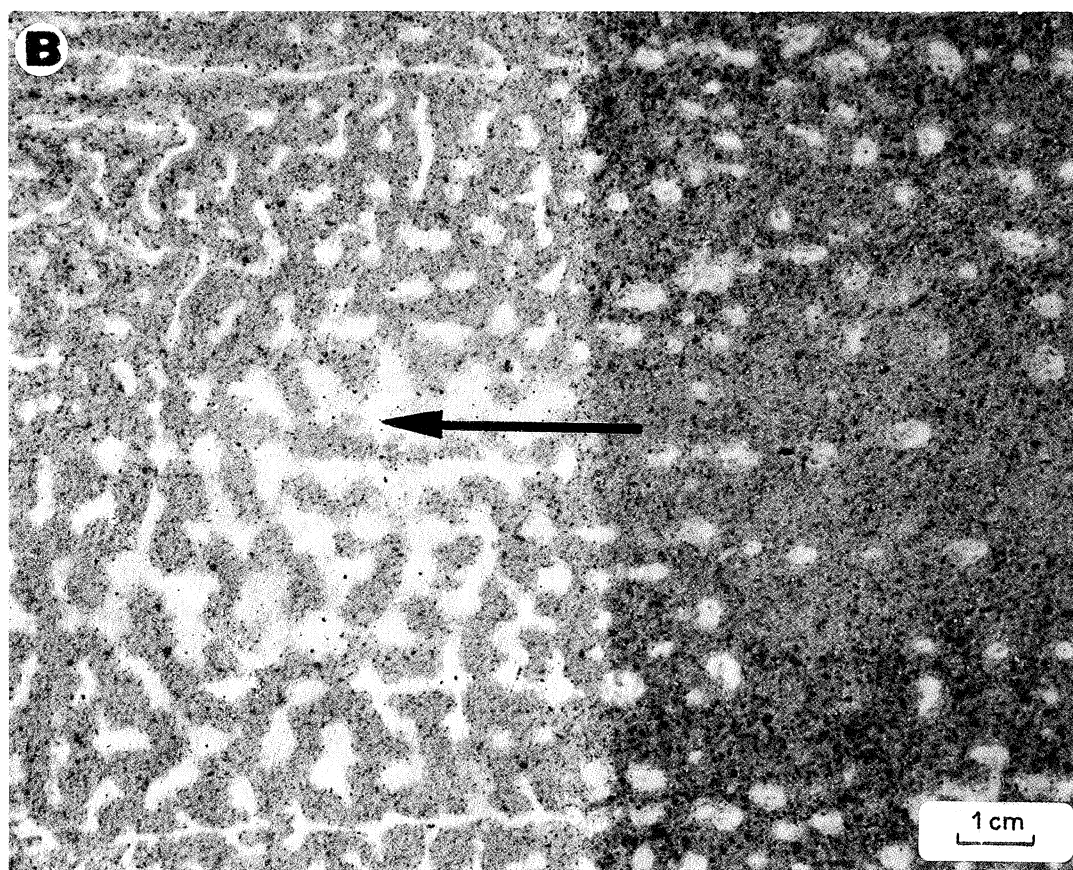
Plate 39 (A) Besko-type convolutions. Oligocene Krosno Beds, Besko. Top view. (B) Experimentally produced deformation pattern similar to that of Besko type convolutions. Explanations in text
