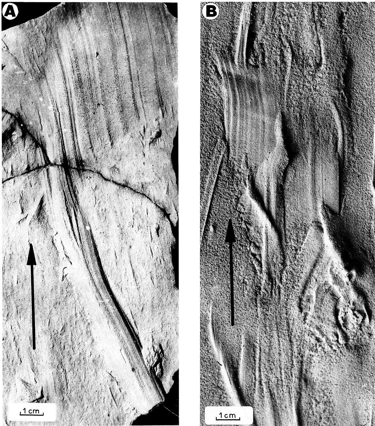
Plate 7 (A) Drag Mark. Upper Mancos Shale, Cretaceous, Black Mesa, California, USA. (B) Experimental drag marks. Base of artificial turbidite (after Dzulynski & Simpson, 1966)
