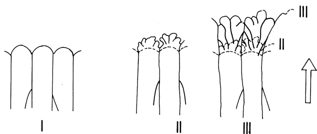
Fig. 26 Schematic diagram showing formations of dendritic ridges by secondary crenulation of lobes of advancing water front. Explanation in text Modified after Dżułyński & Walton (1965)
