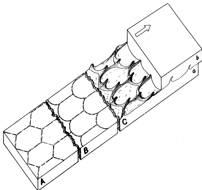
Fig. 20 Transformations of hexahedral pending lobes ( k_a > k_b ) into scales arranged in an en-echelon pattern. After Anketell et al. (1970). Compare Pl. 29. Explanations in text
