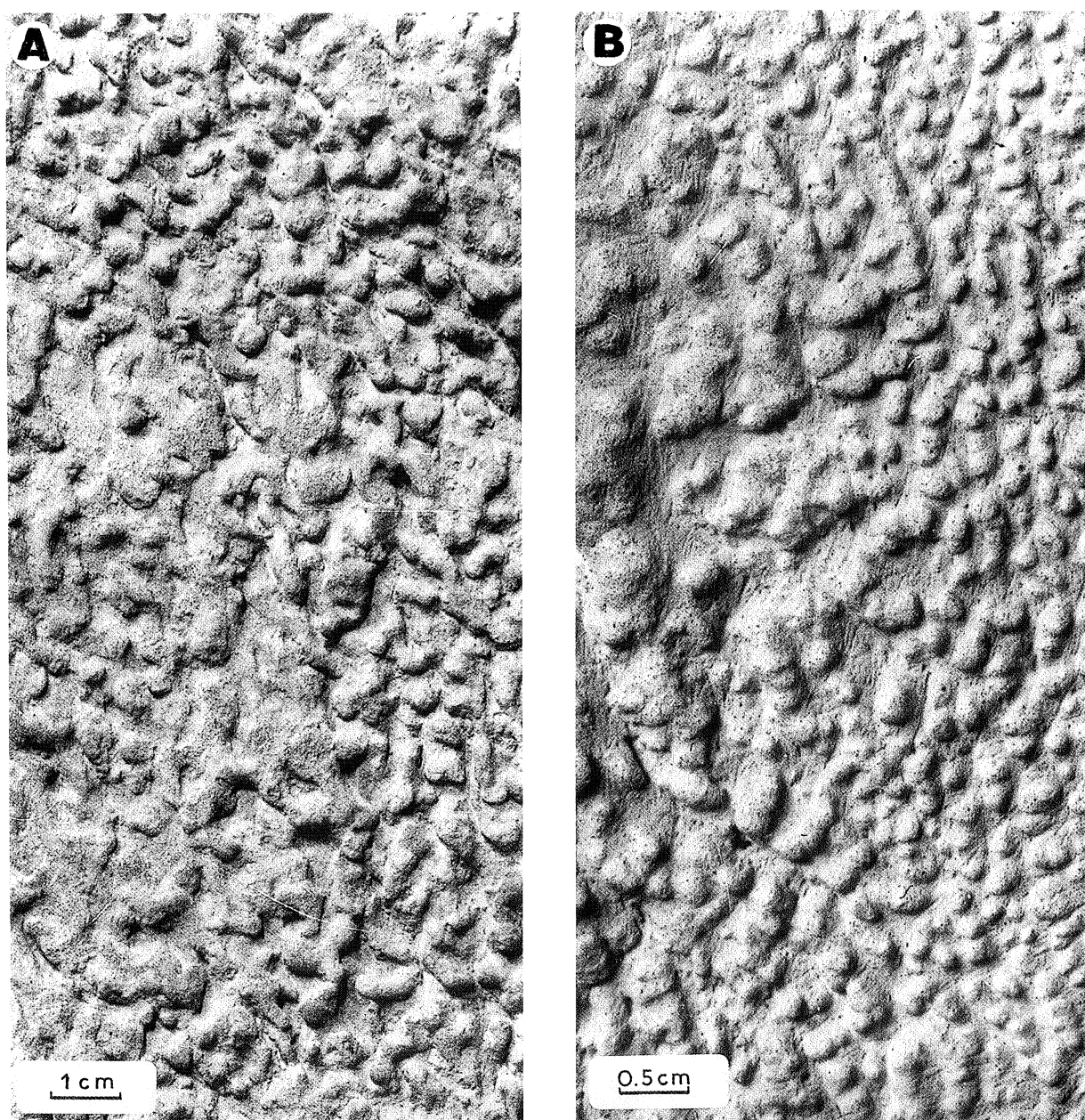
Plate 21 (A) Minor pendulous load deformations. Oligocene Krosno Beds, Rudawka Rymanowska. (B) Minor pendulous load deformations. Base of artificial turbidite
