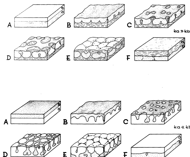
Fig. 10 Selected stages of deformation in non-mobile (ba) systems for different ratios of kinematic viscosities. After Cegla & Dzulynski (1970) and Anketell et al. (1970)
