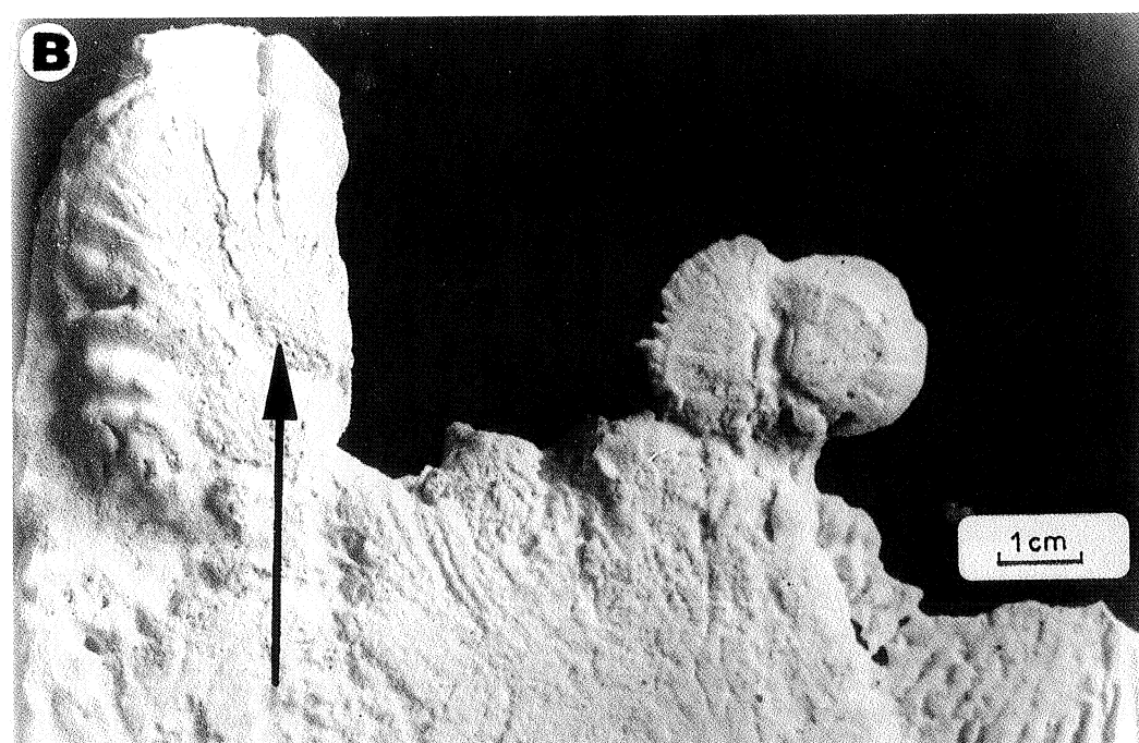
Plate 42 (A) Bulbous frondescent marks. Oligocene Podhale flysch. (B) Bulbous frondescent marks. Experimental structure
