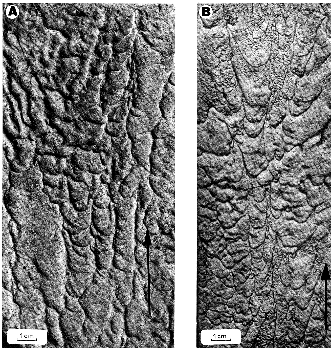
Plate 28 (A) Mixed assemblage of scales arranged in rows and in en echelon pattern. Oligocene Krosno Beds, Rudawka Rymanowska. (B) Mixed assemblage of scales. Base of artificial turbidite
