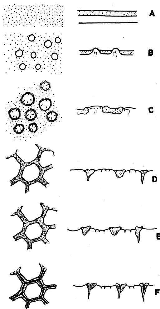
Fig. 12 Formation of polygonal soils from instability in density stratification in plan view ( left ) and cross-section ( right ). Based on experiments. Upper layer; sand and lower clay. After Dzulyński (1963b)
