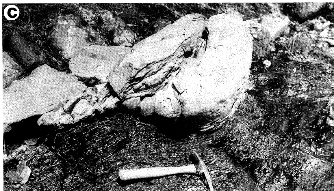
Plate 49 (A), (B) Downward injection of heavy slurry and formation of canoe-shaped structures. Oligocene Magura beds, Ropica Górna. (C) Kidney-shaped clast ripped up and raised by impact of heavy sediment flow. Corrugations on undersurface of covering bed represent moulds of sole markings and moulds of deformed top surface of clast. Cretaceous Inoceranian beds, Ropica Górna
