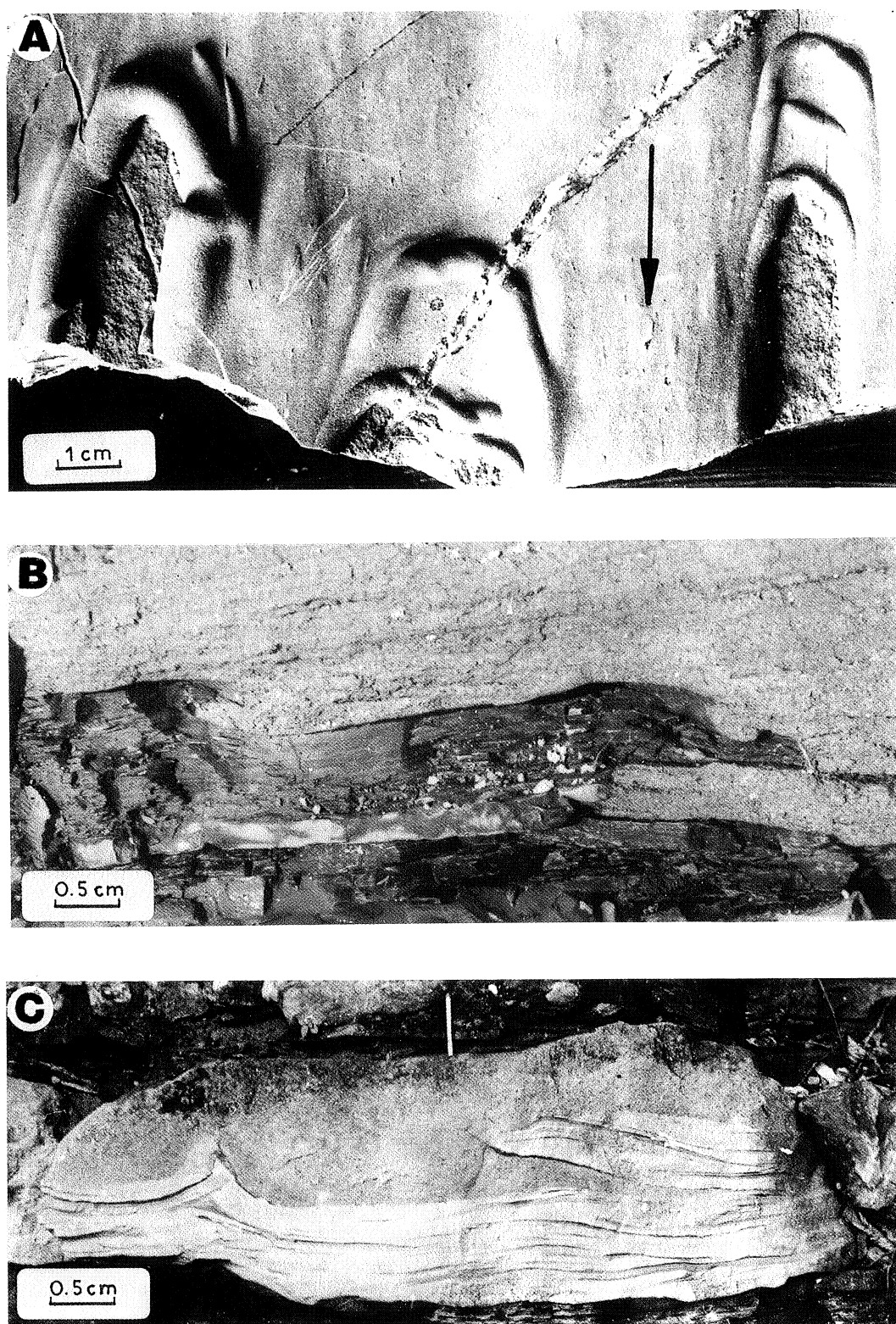
Plate 1 (A) Moulds of crescentic scour marks produced at upcurrent side of resistant patches of lithified shaly intercalation. Successive crescents indicate intermittent retreat of undercut edges of resistant patches. Oligocene Krosno Beds, Wernejowka. Comp. Fig. 1. (B) Undercutting of cohesive bottom mud by strong t-current (sheet flow). Direction of flow is away from observer. Oligocene Magura Beds, Ropica Górna. (C) Incipient uplift of semi-consolidated bottom laminae by downsinking heavy suspension. Detail of amalgamated bed. Direction of flow away from observer. Oligocene Magura Beds, Ropica Górna. Comp. Fig. 35
