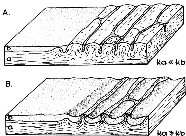
Fig. 18 Schematic presentation of deformation pattern in non mobile (ba) system in which instability propagates laterally. Direction of propagation shown by arrow. After Anketell et al. 1970
