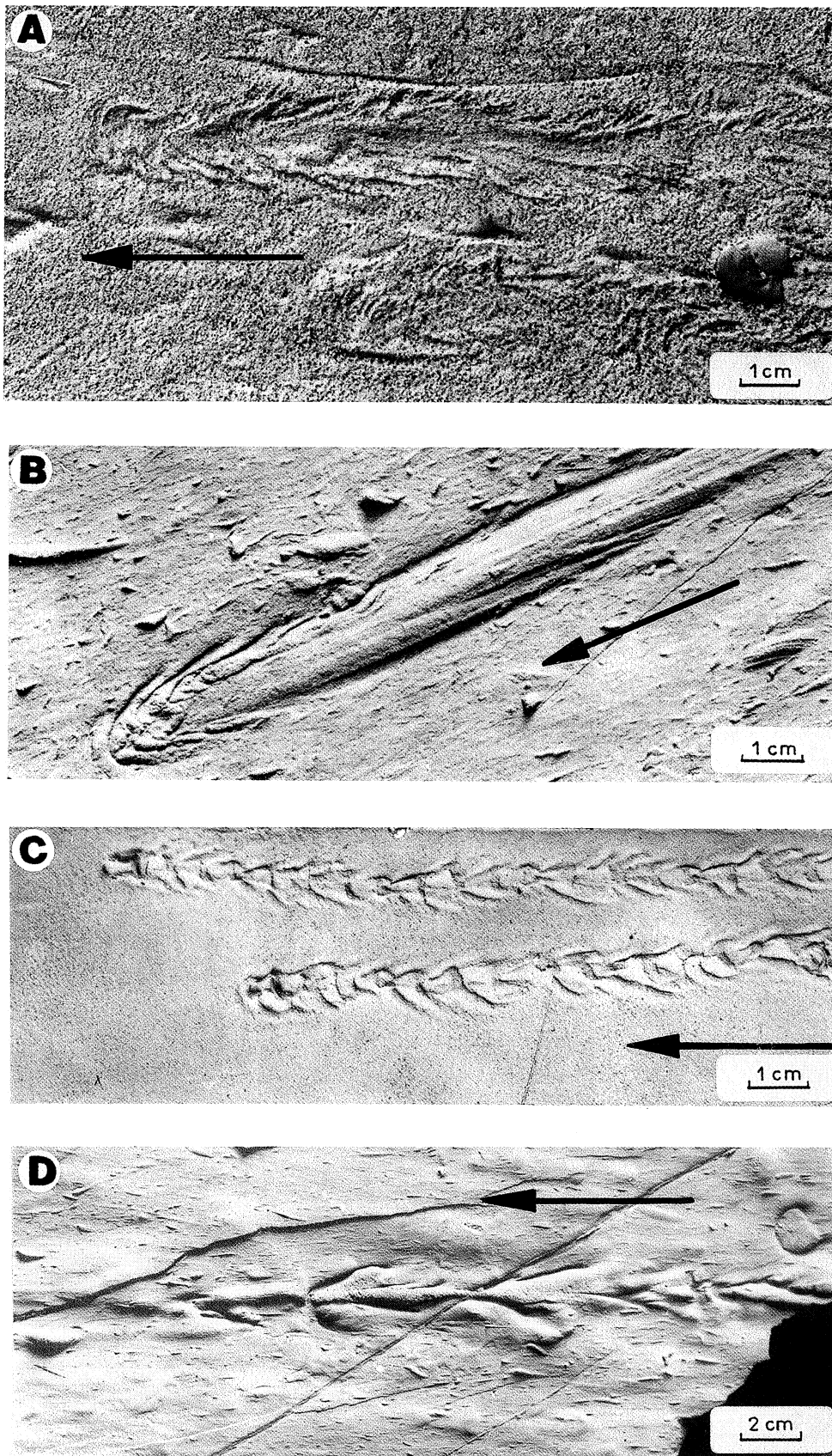
Plate 9 (A) Doubly ruffled groove. Base of artificial turbidite (after Dzulynski & Simpson, 1966). (B) Partly double ruffled groove. Oligocene Krosno Beds, Rudawka Rymanowska. (C) Chevron mark produced by skimming fish vertebrae. Base of artificial turbidite. (D) Chevron mark produced by skimming fish vertebra. Oligocene Krosno Beds, Kały
