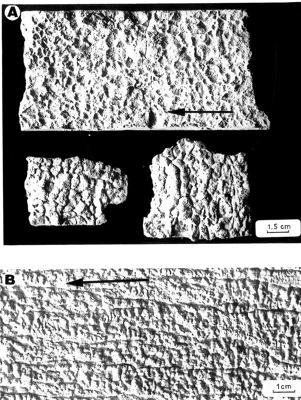
Plate 31 (A) Experimental transverse and polygonal scaly structure. Upper picture shows “positive” and lower “negative” aspects of same structure. (B) Transverse structures between moulds of longitudinal ridges. Base of artificial turbidite
