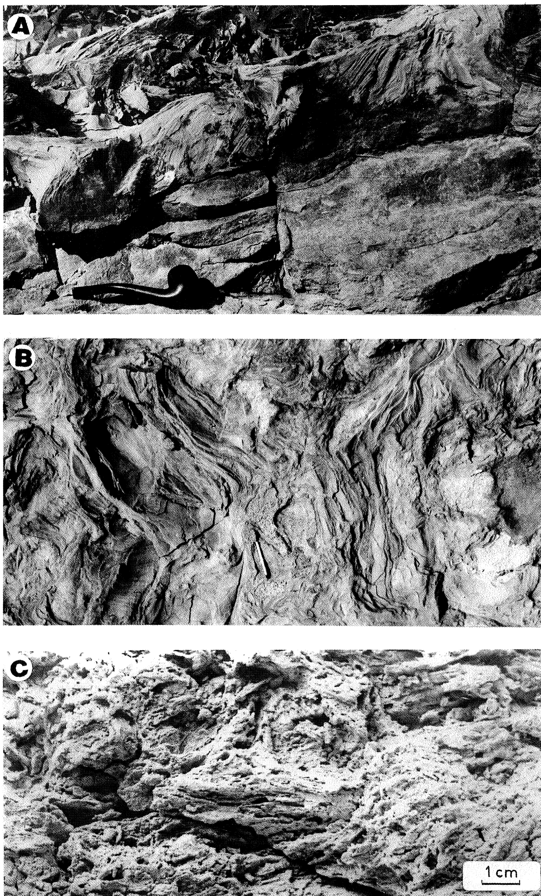
Plate 43 Crinkled lamination on top of massive sandstone. (A - side view; B - top view). Oligocene Magura beds, Bednarka. (C) Experimental crinkled lamination. Top view
