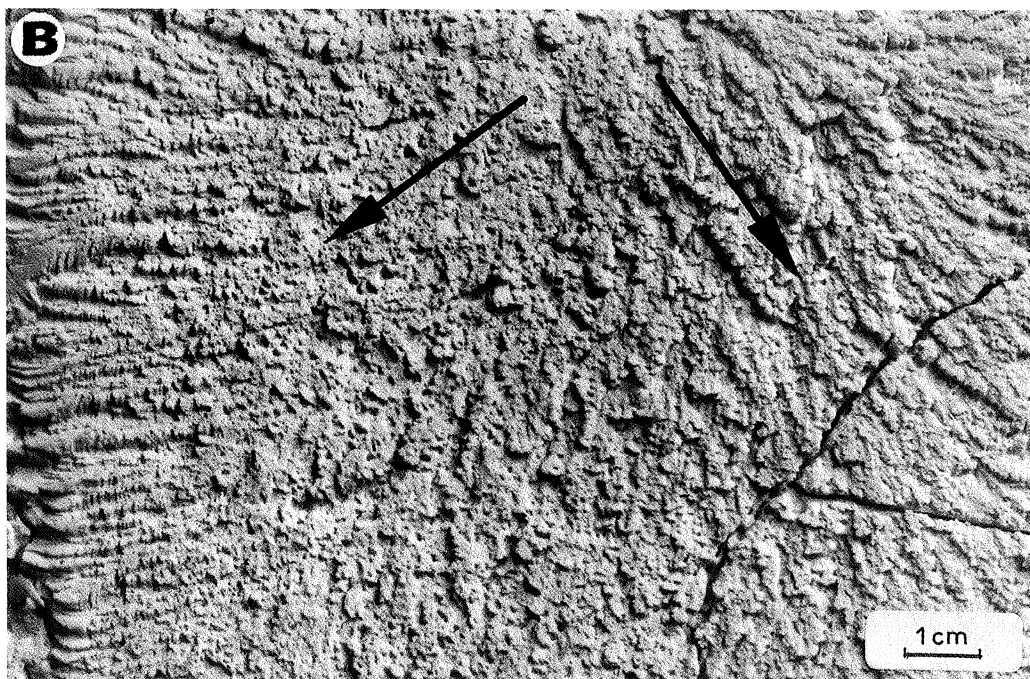
Plate 41 (A) Frondose marks. Oligocene Krosno beds, Rudawka Rymanowska. (B) Experimental frondose markings (after Dżułyński & Walton 1965)
