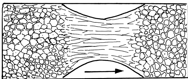
Fig. 25 Polygonal ridges and scales passing into l-ridges in narrow passage of flume. After Dżułyński & Simpson (1966b)
