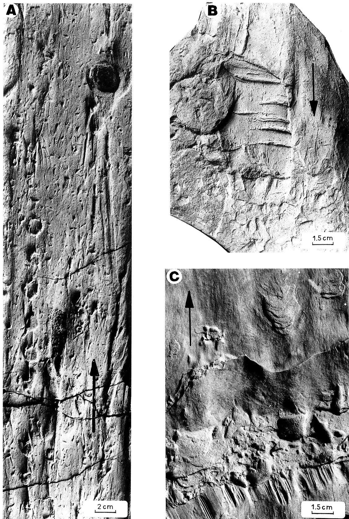
Plate 2 (A) Discoidal shale fragment at downcurrent end of groove mould. Oligocene Menilite Beds, Rudawka Rymanowska. (B) Mould of fractured shale fragment at downcurrent end of groove mark. Transverse ridges represent infillings of open fractures by settling sand. Oligocene Podhale Flysch, Witów. (C) Mould of brush mark produced by impact of large shale fragment with moulds of smaller pieces of shale detached from margins of impinging fragment on collision with bottom. Oligocene Krosno Beds, Besko
