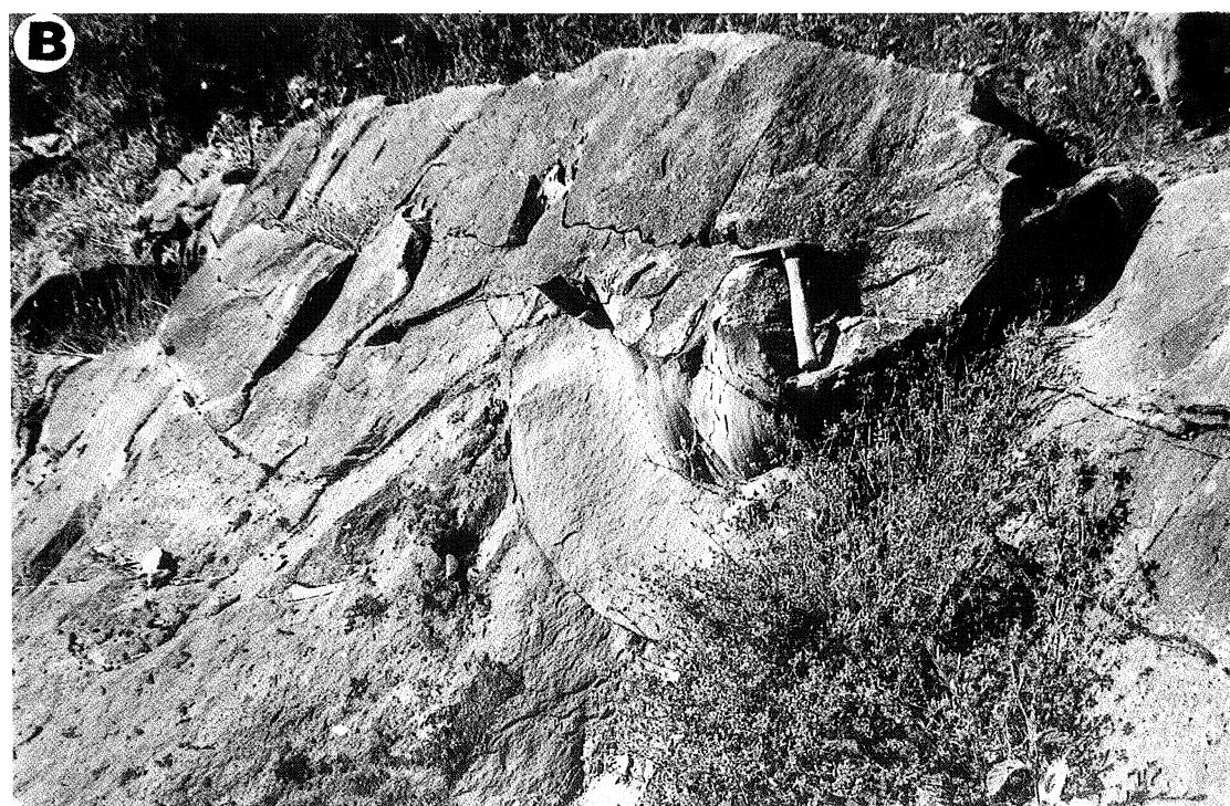
Plate 38 (A) Ridged convolutions in dichotomous bed whose lower member is horizontally laminated and upper one rippled. Oligocene Krosno Beds, Mymoń. (B) Ridged convolutions in laminated sandstone. Oligocene Krosno Beds, Sieniawa
