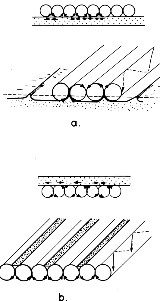
Fig. 24 Schematic presentation of development of experimentally produced current ridges (a) and sorted stripes (b). After Dżułyński & Walton (1963), Dżułyński (1966). Explanations in text
