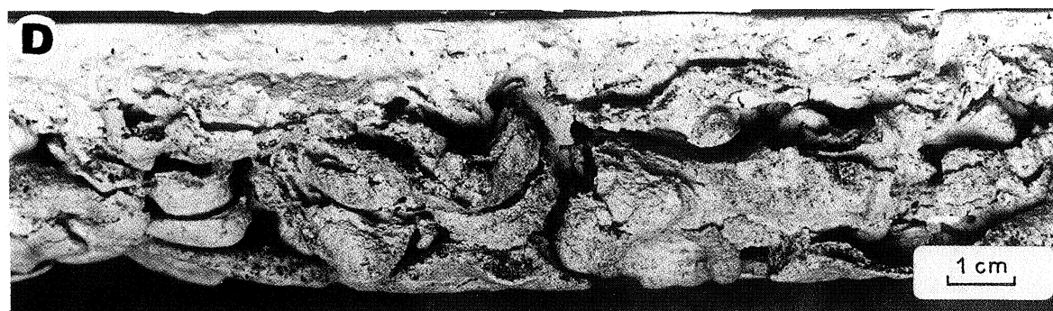
Plate 47 (A) Experimentally produced prolapse fold (after Dżułyński & Radomski, 1966). (B) Flow parallel longitudinal folds. Base of heavy sediment flow deposited upon layered substratum. Base of experimental flow deposit (after Dżułyński & Radomski, 1966). (C) Transverse section of experimental longitudinal folds. (D) Transverse cross-section of longitudinal structures produced by flow of heavy suspension upon stratified substratum. Experimental structure
