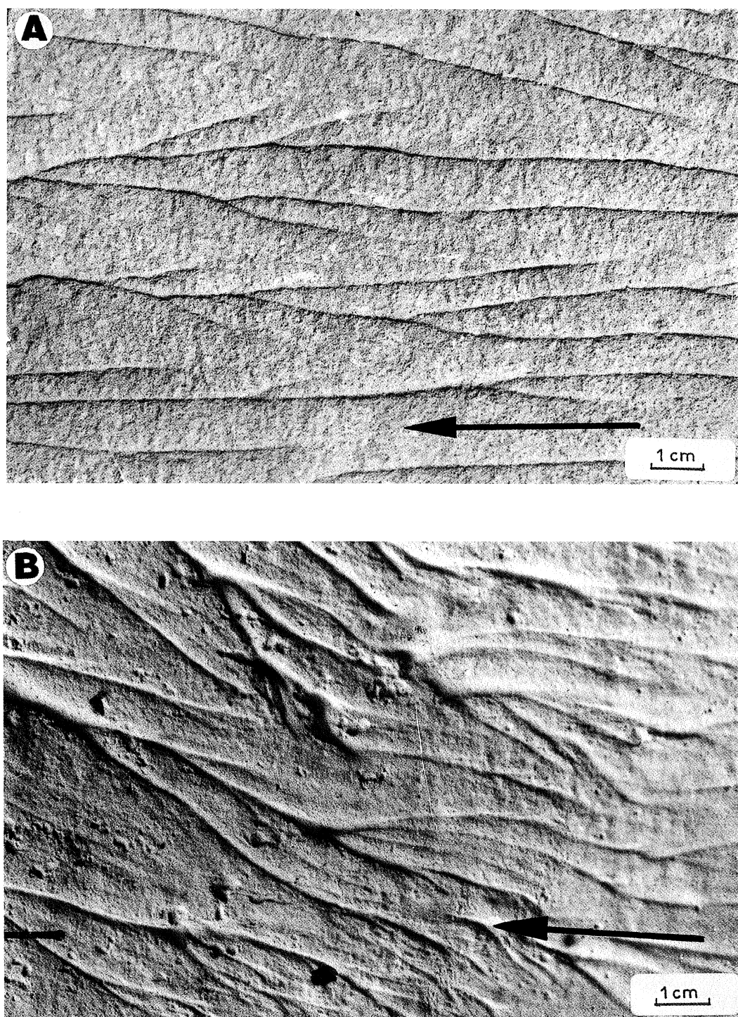
Plate 33 (A) Moulds of dendritic ridges. Oligocene Krosno beds, Mokre. (B) Experimentally produced dendritic ridges. Explanation in text
