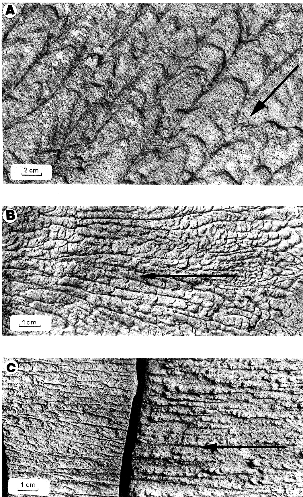
Plate 26 (A) Scales arranged in flow-parallel rows. Oligocene Magura Beds, Ropica Górna. (B) Scales arranged in flow-parallel rows. Base of artificial turbidite (after Dzulynski & Simpson, 1966). (C) Positives of experimental scales arranged in flow-parallel rows. Explanation in text (after Dzulynski & Simpson, 1966)
