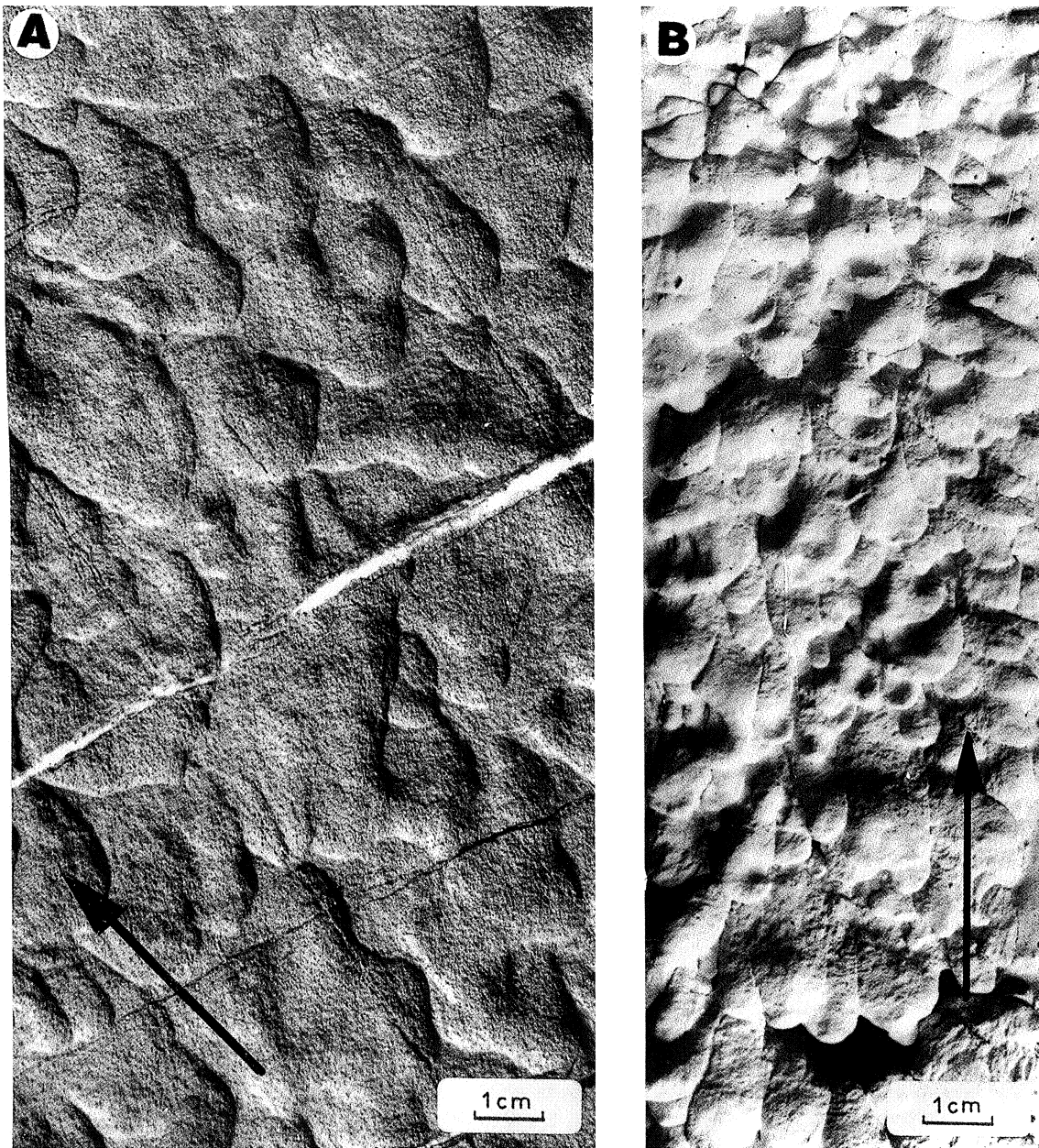
Plate 27 (A) Scales arranged in en echelon pattern. Oligocene Krosno Beds, Rudawka Rymanowka. (B) Scales arranged in en echelon pattern. Base of artificial turbidite (after Dżułyński & Walton 1965)
