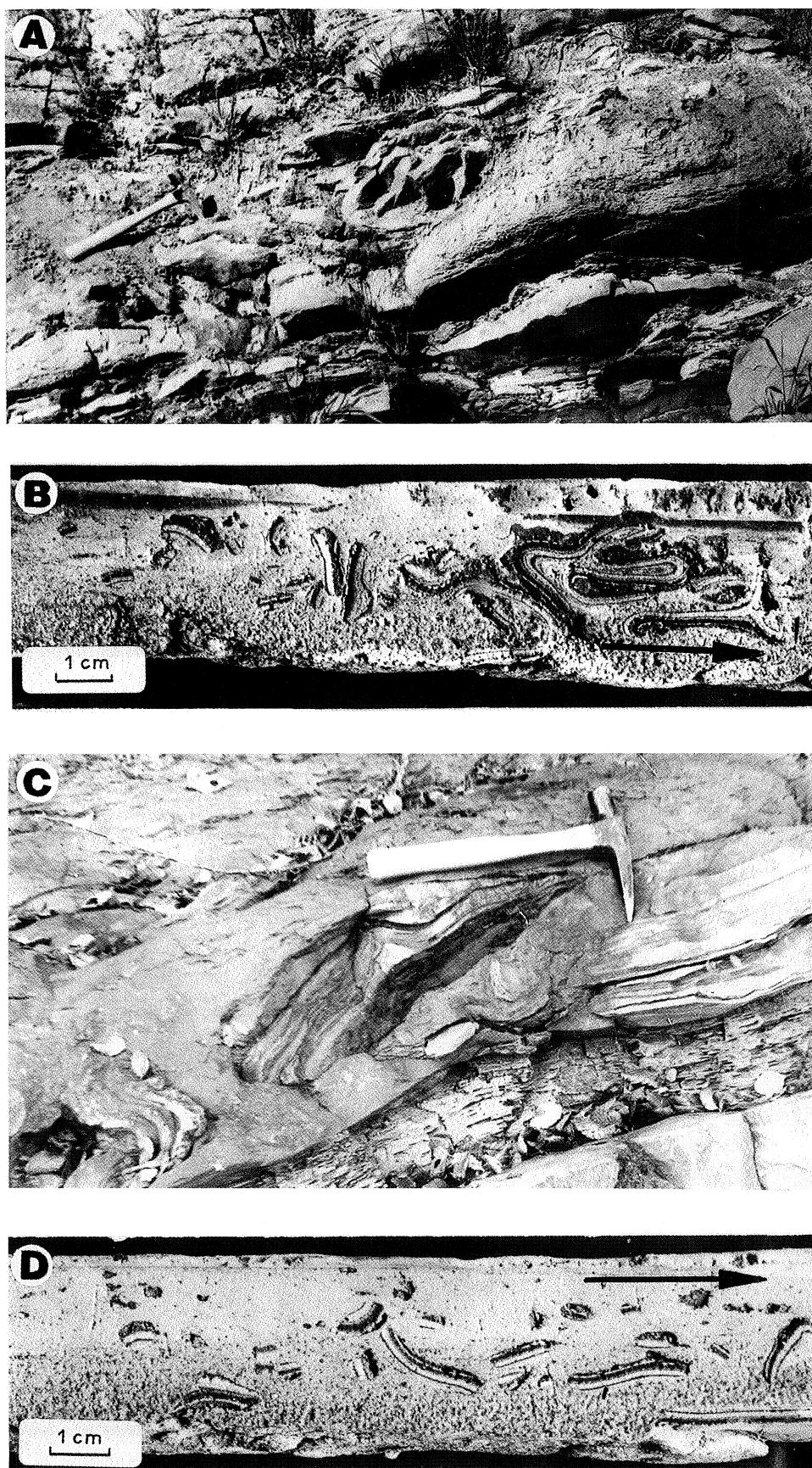
Plate 46 (A) Contorted pack of ripped-up layers in sediment-flow deposit. Oligocene Magura beds, Ropica Górna. (B) Analogous structure produced experimentally. (C) Angular clasts incorporated into sediment flow. Oligocene Magura beds, Ropica Górna. (D) Analogous structure as above produced experimentally
