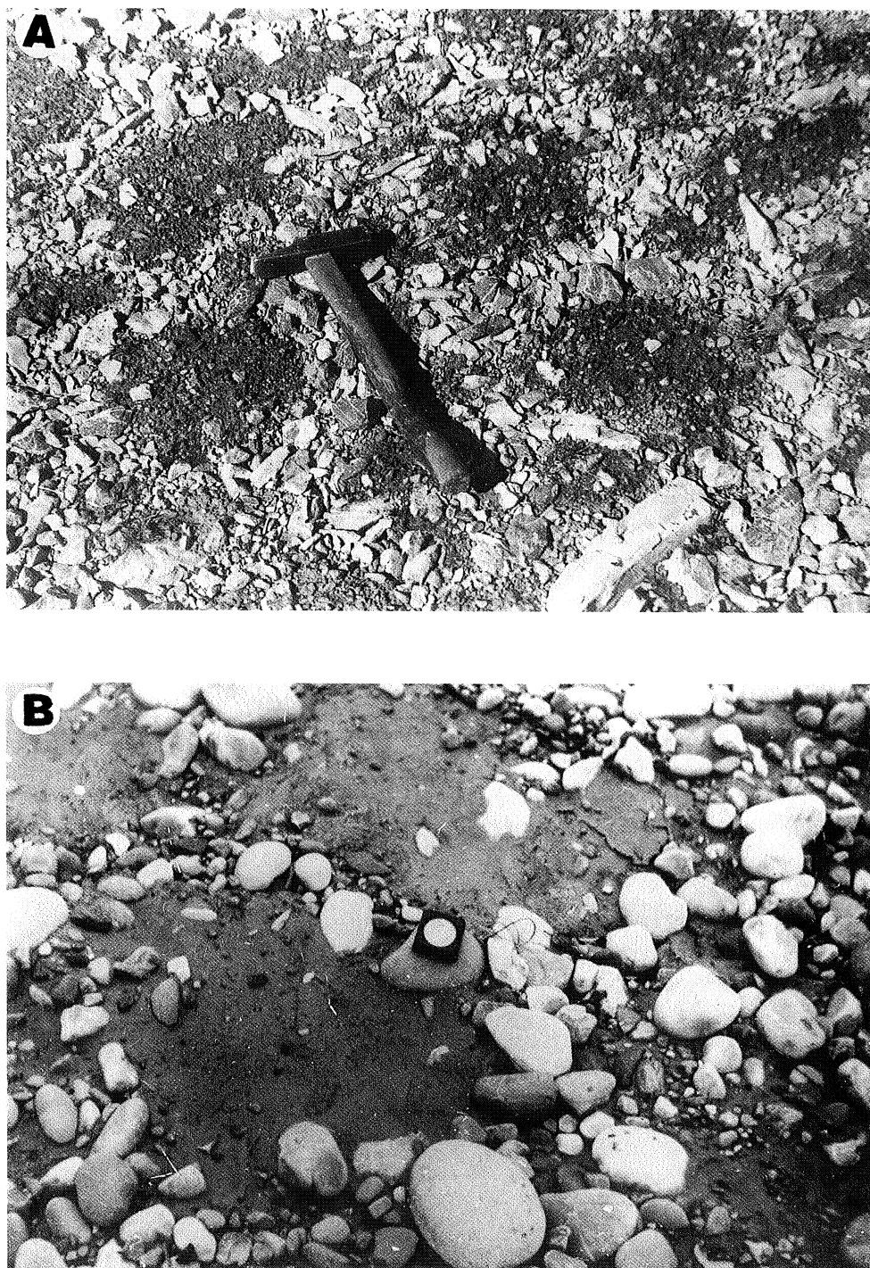
Plate 24 (A) Sorted polygons in periglacial environment. Engadin, Alps, Switzerland. (B) Sorted polygons in subtropical environment. Sivaliks, India (after R. Soja, in preparation)
