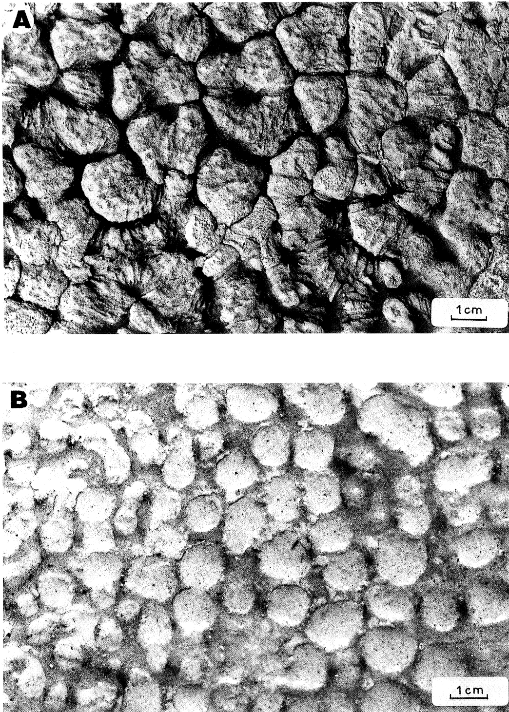
Plate 23 (A) Surface of rising columns of lower member (a) before they reached top surface of non mobile (ba) system. Experimental structure. (B) Experimental sorted polygons and sorted circles on top surface of non mobile (ba) system (after Cegla & Dzułyński, 1970)
