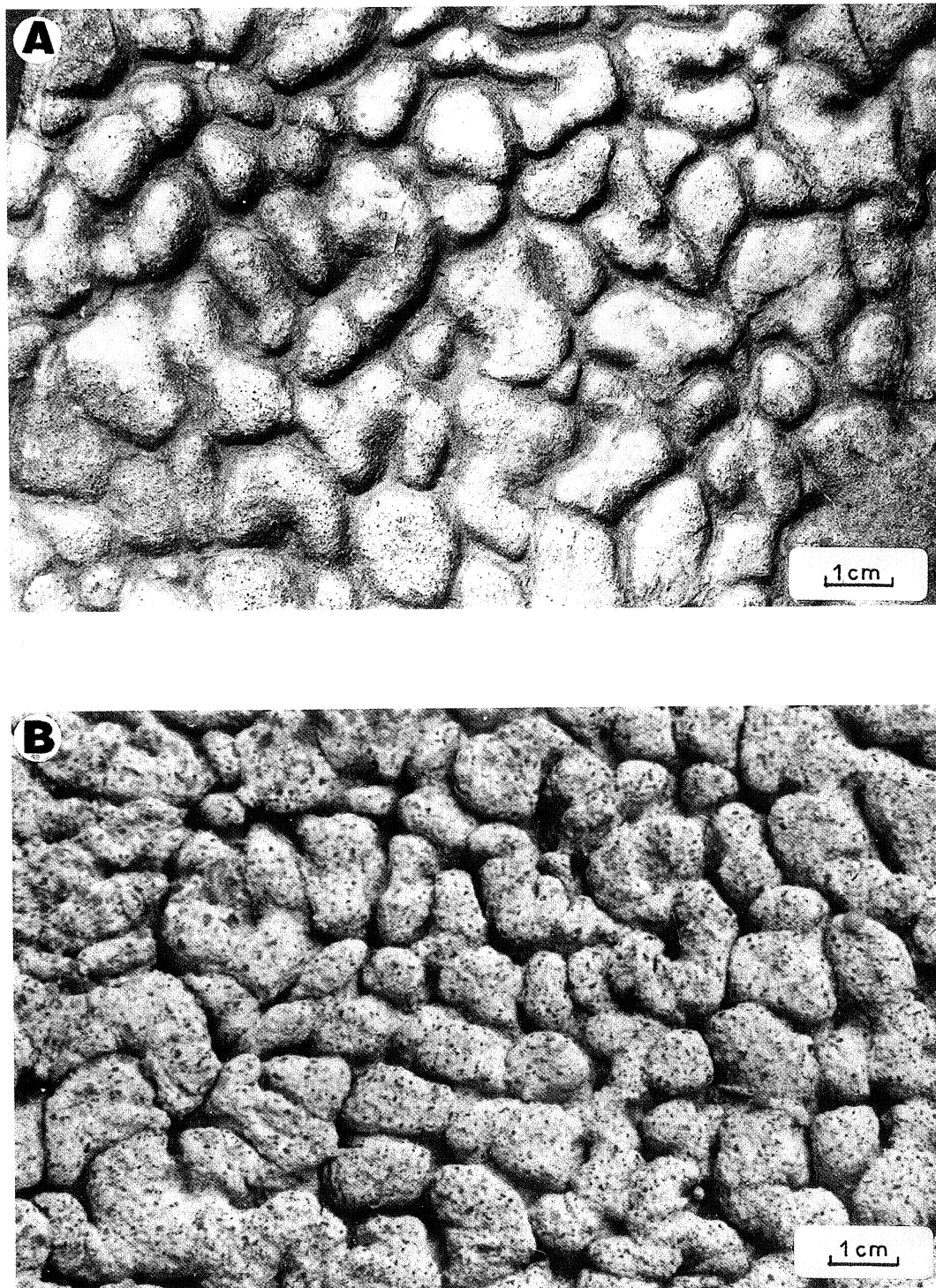
Plate 19 (A) Polygonal load casts. Oligocene Krosno Beds, Rudawka Rymanowska. (B) Polygonal load casts. Base of artificial turbidite (after Dzulynski & Simpson, 1966)
