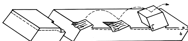
Fig. 28 Diagram showing impact induced dendritic ridges. Comp. Pl. 11C. After Dżułyński et al. 1972
