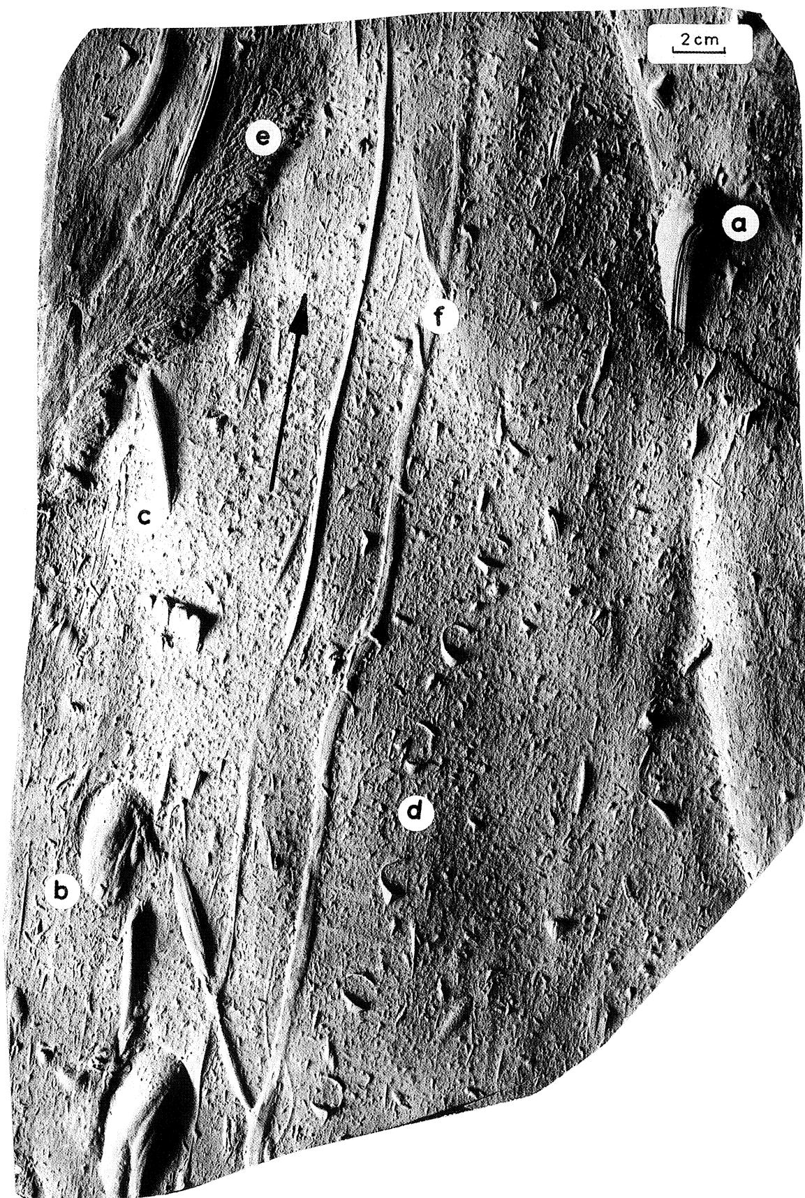
Plate 4 Base of sandstone with moulds of: (a) prod marks, (b) brush marks, (c) bounce marks, (d) saltation marks of fish vertebrae, (e) frondescent mark, (f) double groove mould. Oligocene Krosno Beds, Wetlina
