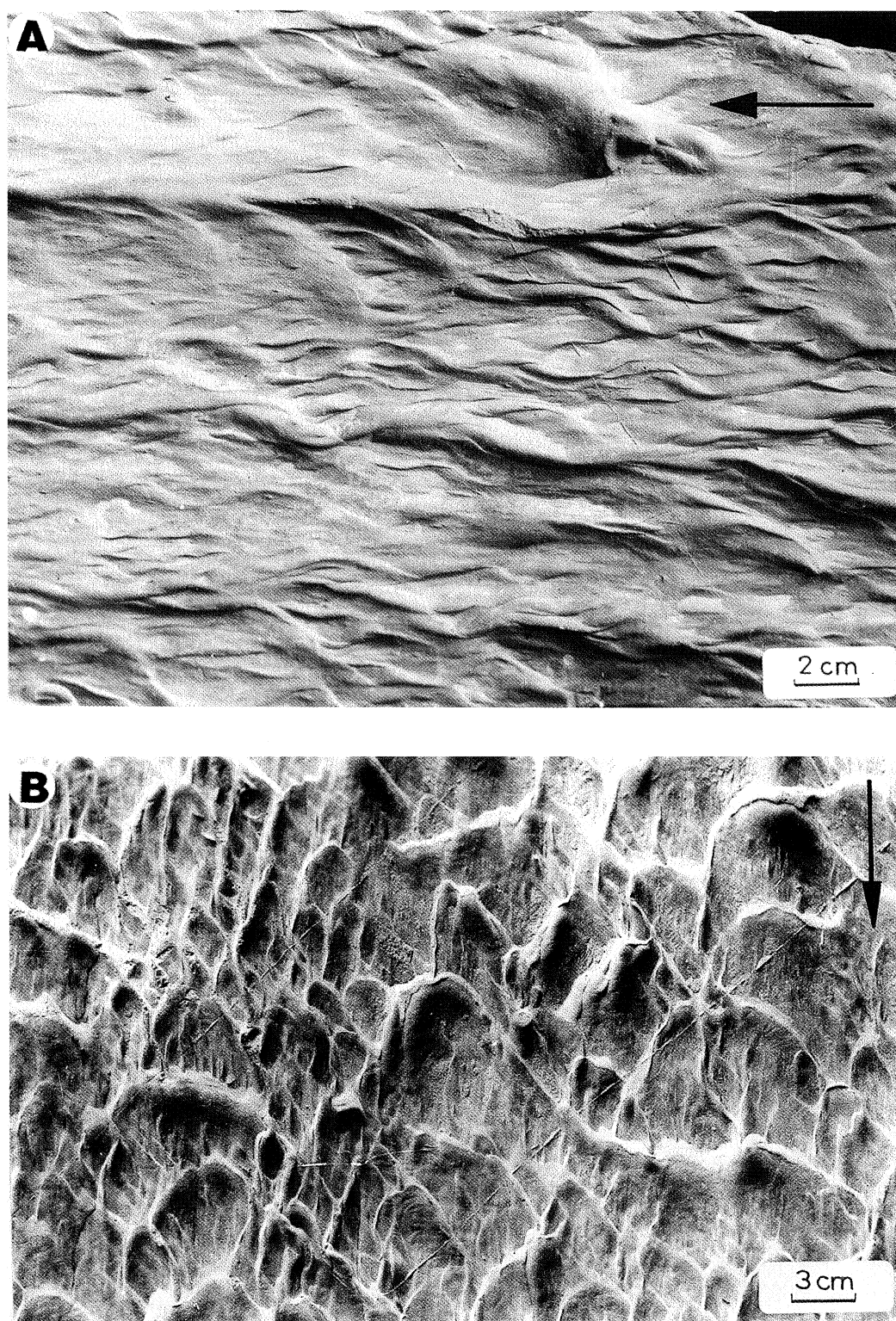
Plate 16 (A) Slightly meandering moulds of rill markings. Oligocene Krosno Beds, Wernejówka. (B) Rill markings arranged in diagonal pattern. Oligocene Krosno Beds, Wernejówka
