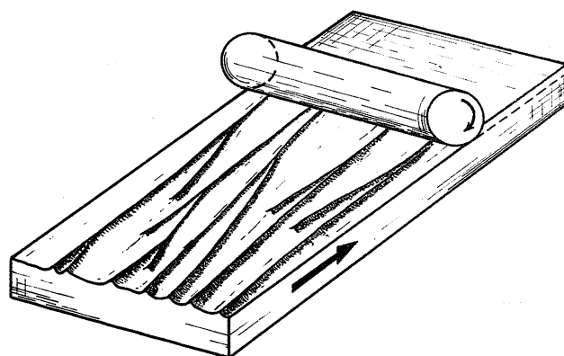
Fig. 27 Diagram showing formation of dendritic ridges by rolling cylinder
