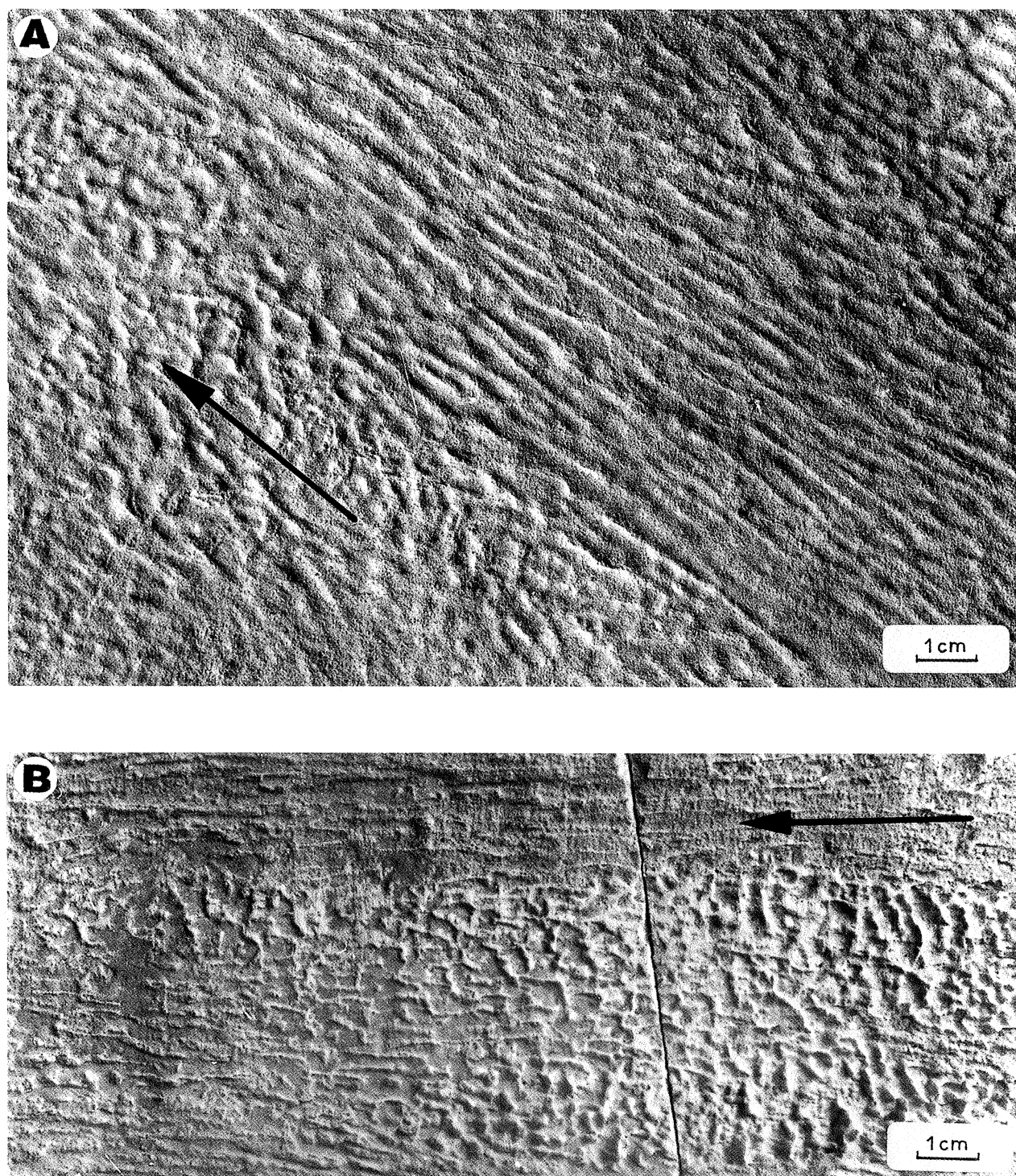
Plate 36 (A) Top of parting surface of sandstone bed showing alternating zones of longitudinal and polygonal ridges. Oligocene Menilite Beds, Wetlina. (B) Positives of alternating longitudinal and polygonal ridges. Experimental structures (after Dzulynski & Simpson, 1966)
