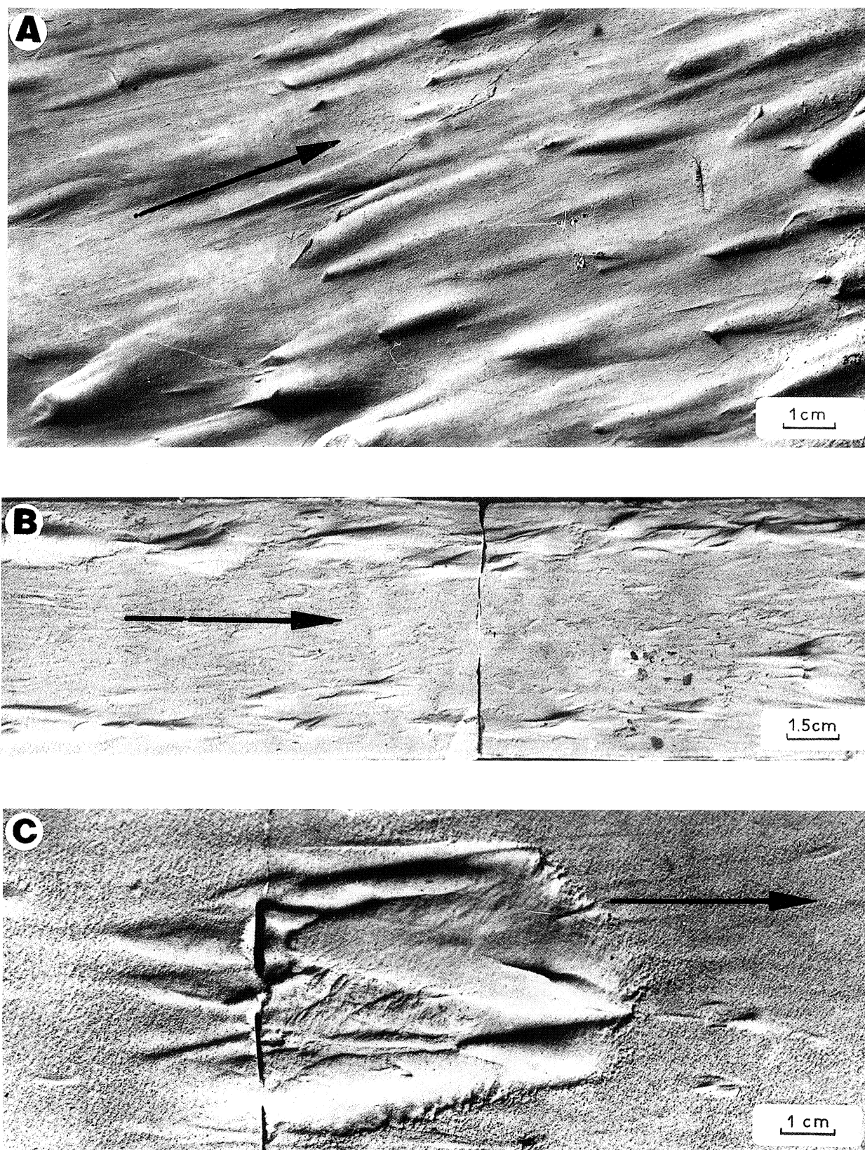
Plate 13 (A) Flute markings at downcurrent ends of prod markings. Oligocene Krosno Beds, Rudawka Rymanowska. (B) Flute moulds at downcurrent ends of prod markings. Base of artificial turbidite (after Dzulynski & Simpson, 1966). (C) Relatively large flute moulds at downcurrent ends of prod marks. Note prod mark with smaller flute superimposed upon large flute. Base of artificial turbidite (after Dzulynski & Simpson, 1966)
