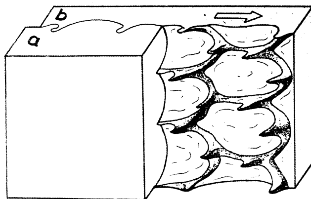
Fig. 22 Transformations of hexahedral up-rising domes ( k_a < k_b ) into scales arranged in an en-echelon pattern. After Anketell et al. (1970). Explanations in text
