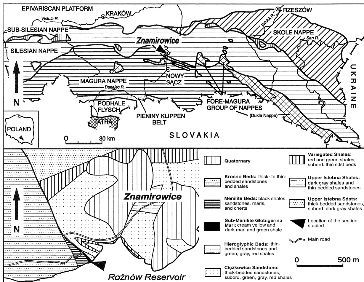
Fig. 1 Location of the examined section. A. Location of the section relative to regional geology. B. Location of the section at Znamirówice
