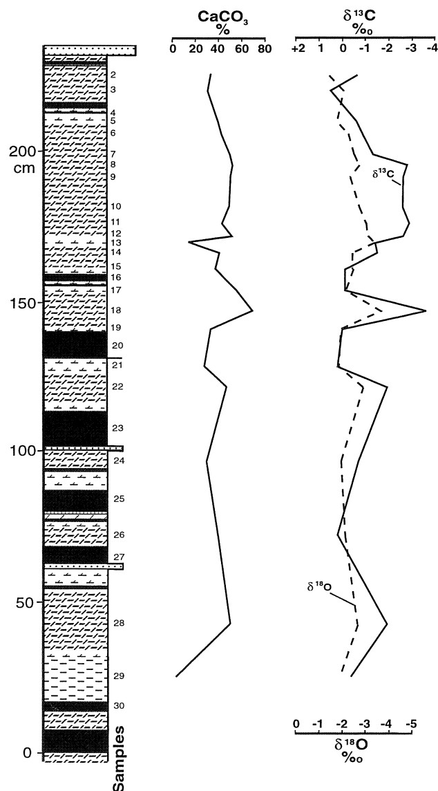
Fig. 21 Relationships between \text{CaCO}_3 content, \delta^{18}\text{O} , and \delta^{13}\text{C} in light marls and green shales
