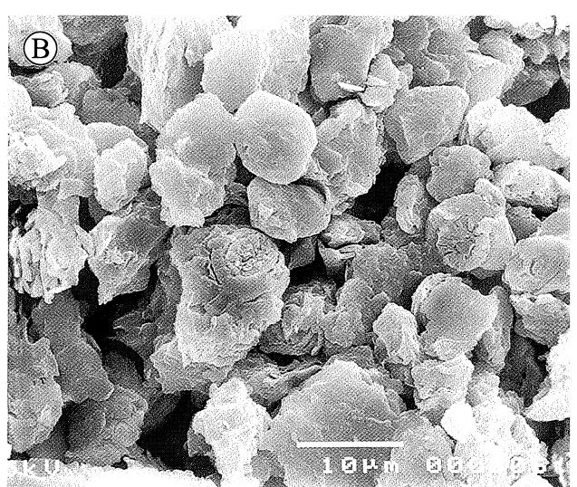
Fig. 18 Nannofossils in smear slides. A. Highly calcareous marl (sample 8); B. Dark-brown shale. Note single, highly corroded and recrystallized specimens (sample 4)
