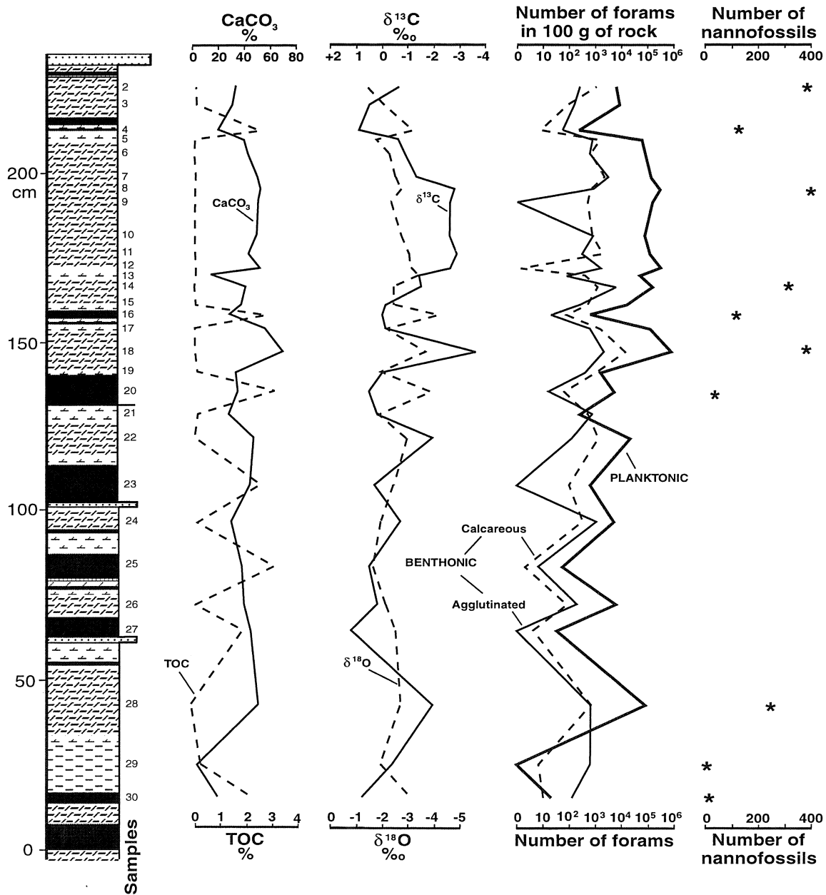
Fig. 11 TOC, CaCO 3 , C and O stable isotopes, foraminifera and nannoplankton signals in upper part of the SMGM package at Znamirówice
