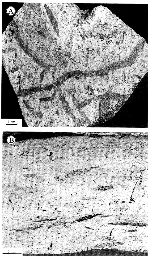
Fig. 8 Bioturbation in greenish marl overlain by thin lamina of dark-coloured marl. Burrows are accentuated by dark colour of their fill. A. View on bedding-parallel fracture surface; B. View in vertical cross-section. Note inverse grading of burrow concentration towards the layer top
