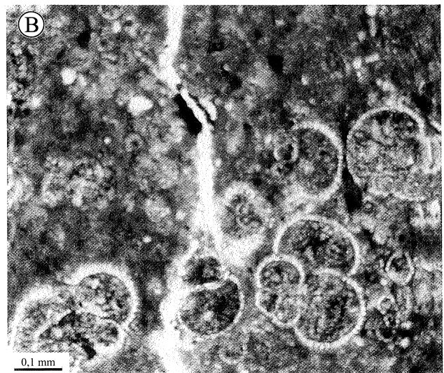
Fig. 13 Concentration of planktonic foraminifera in the light-coloured marl (sample 7). A. Irregular distribution of sediment constituents; B. Different preservation of foraminifera tests
