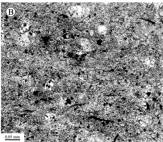
Fig. 17 Microfeatures of the light-coloured marl of the Sub-Chert Beds. At same magnification as in Figs. 13A, 15, 16, it appears that foraminifera are absent in this sediment. A. Only single, larger foraminifera appear at this magnification; B. Significantly higher amount of foraminifera is visible at a higher magnification. Note the common occurrence of pyrite (black) in chambers of foraminifera tests and the parallel arrangement of elongated grains (mica flakes and coalified plant fragments)
