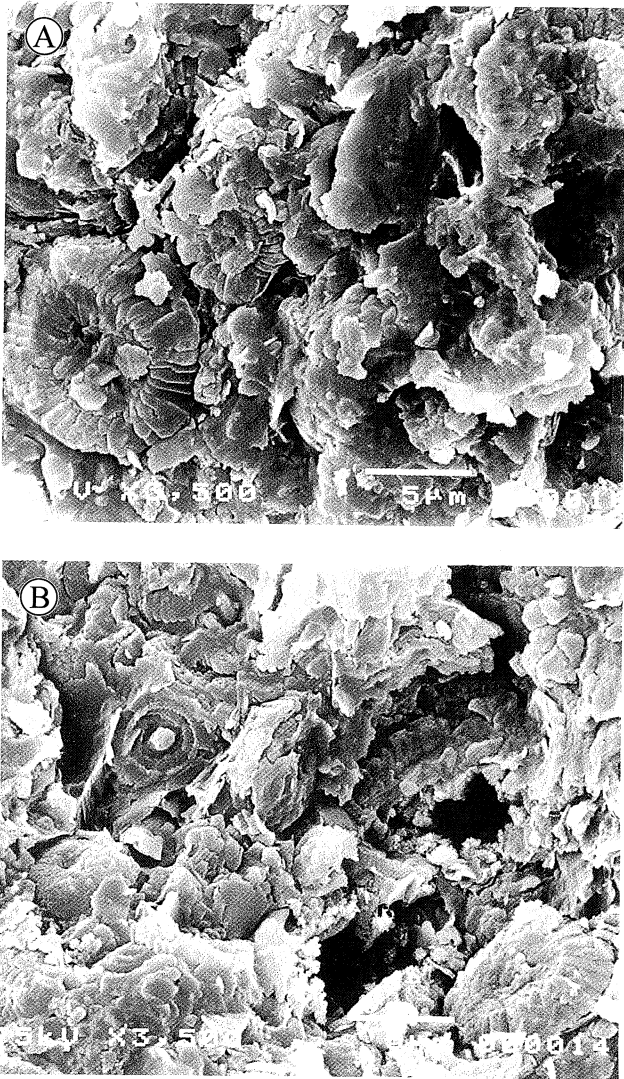
Fig. 19 Nanofossils in hard marl. Note the poor preservation, overgrowth and recrystallization of specimens (sample 8); A . Specimen to the right of the centre disappears in newly formed mineral matter; B . Concentration of highly altered nanofossils
