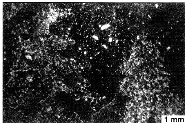
Fig. 8. Boundstone-bafflestone, locally wackestone. A fragment of siliceous sponge with numerous leiolites; nodular limestones, Ostatnia Cliff
