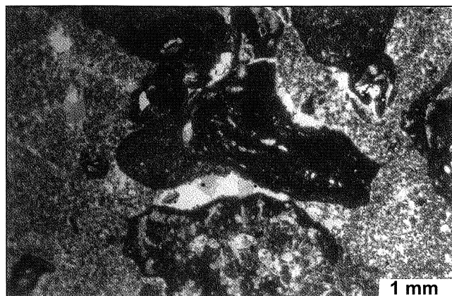
Fig. 10. Wackestone – floatstone with “ Tubiphytes ” morronensis ; Księża Hill
