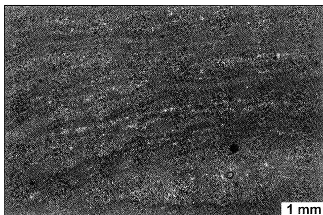
Fig. 9. Boundstone micritic stromatolites. Zakrzówek Quarry
