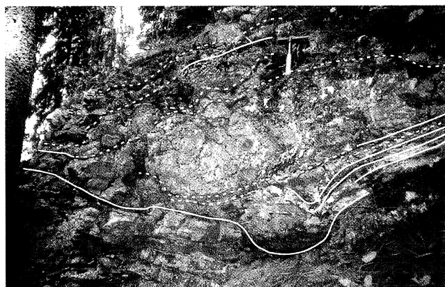
Fig. 5. Submarine slump within the studied spiculites; note uneven base of the slumped beds; Huciański Klin crest
