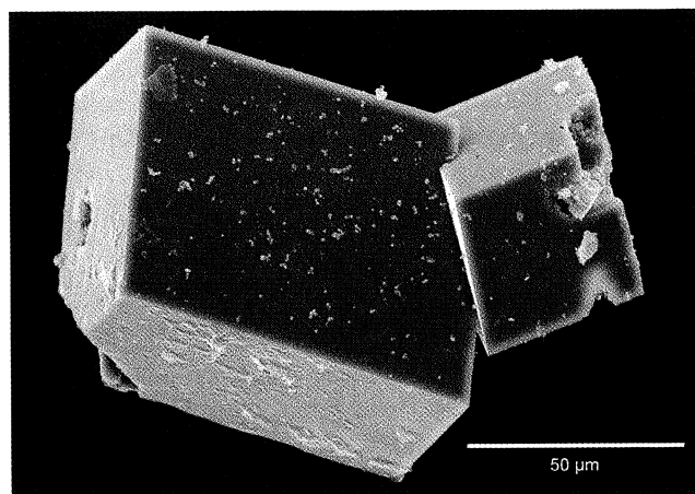
Fig. 12. Calcite rhombohedra isolated by HF etching; SEM image; Zadnia Kopka hill
