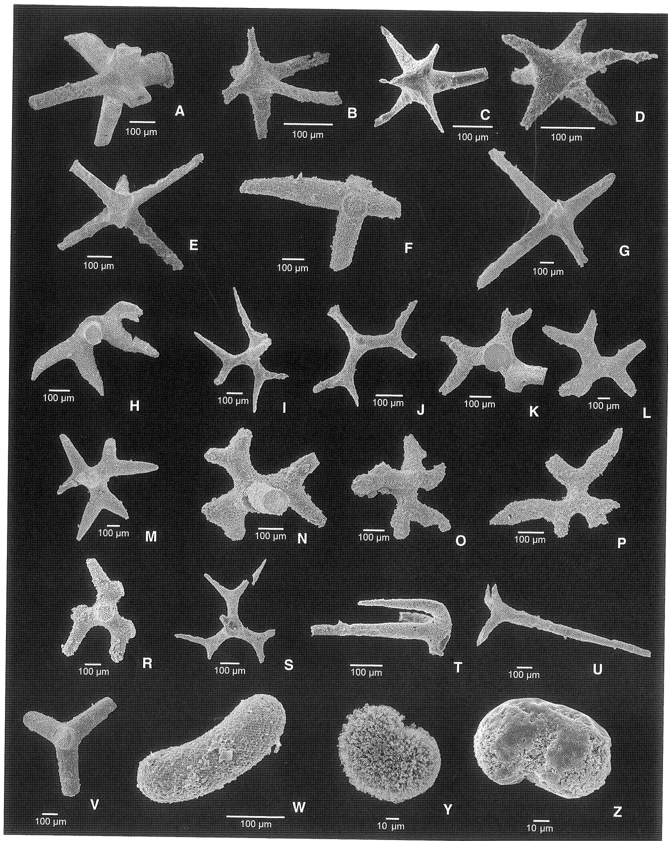
Fig. 8. Selected spicules isolated by etching in HF. Hexactinellid spicules: A–G. hexactines; Demosponge spicules: H–S. dichotriaenes; T. anatriaene; U. triaene; V. tetractine; W. strongyle; Y–Z. selenasters
