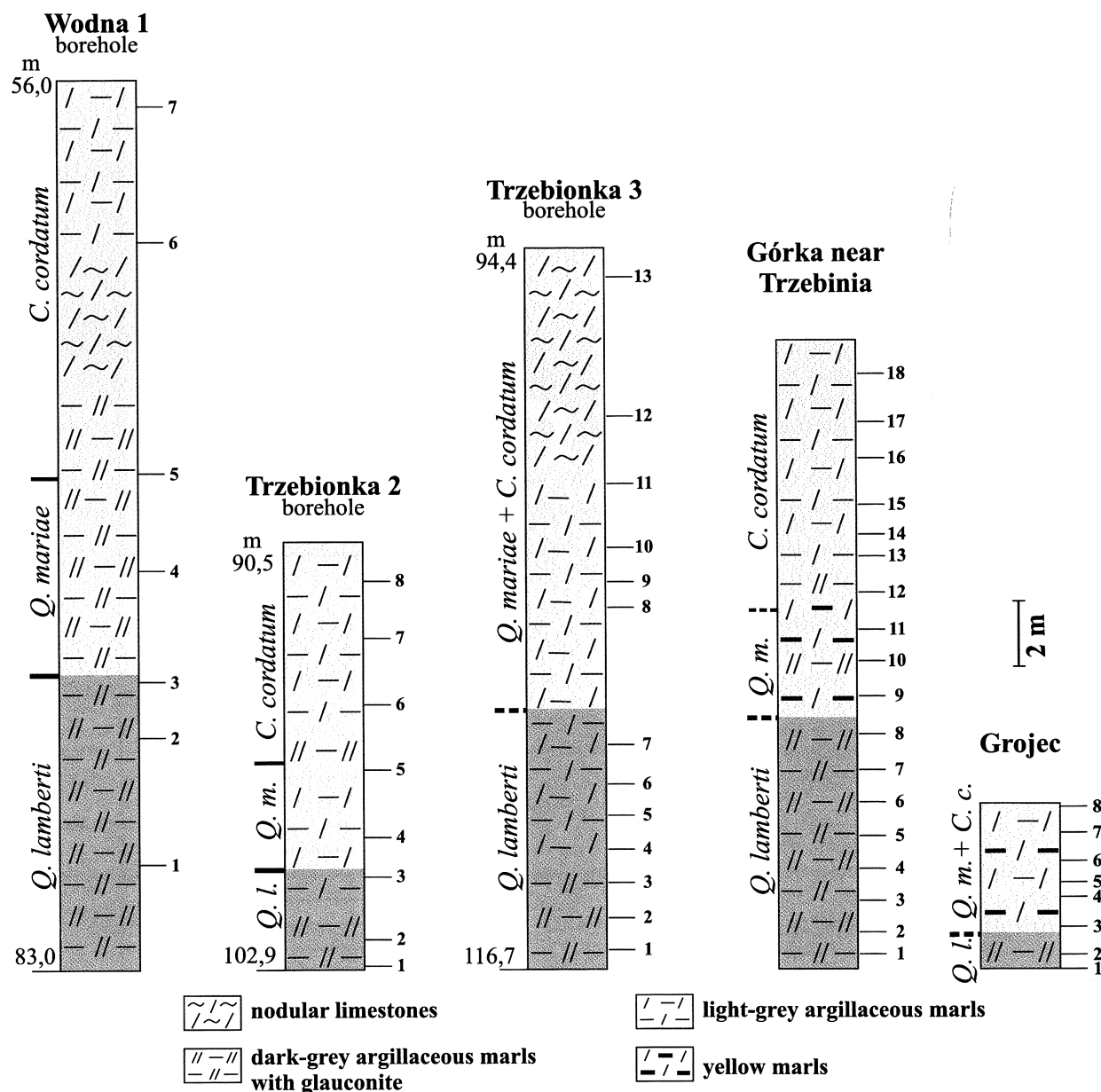
Fig. 3. Lithostratigraphical profiles of the studied sections in the Kraków-Wieluń Upland (after Malinowska, 1991; Różycki, 1953), with the positions of the radiolarian samples. Q. l – Quenstedtoceras lamberti Zone (grey background of signatures); Q. m – Quenstedtoceras mariae Zone; C. c – Cardioceras cordatum Zone. Scale bar – the same for all profiles
