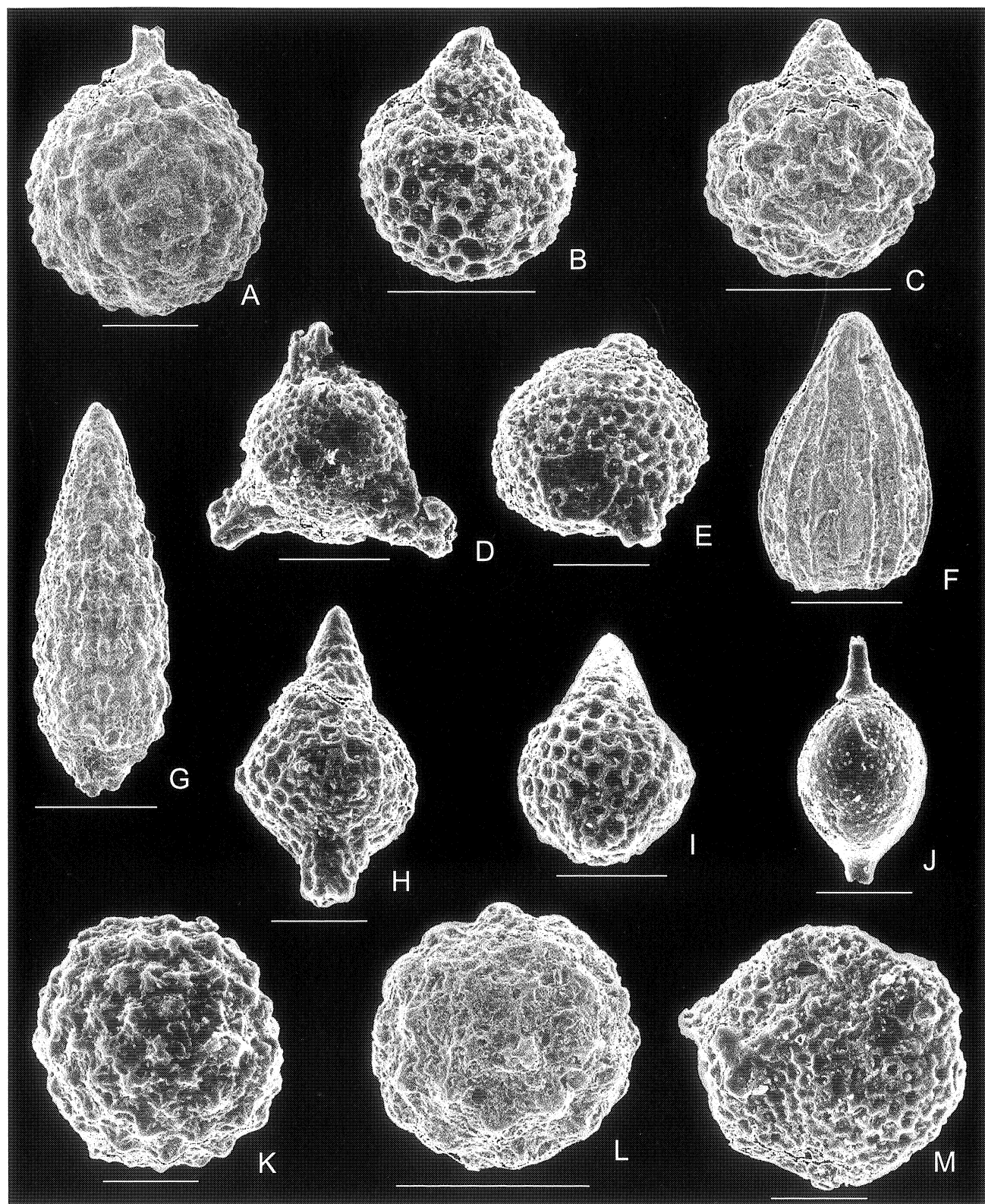
Fig. 12. Upper Callovian radiolarians from the Górka near Trzebinia outcrop and from the Trzebionka 3 borehole (Kraków–Wieluń Upland) – assemblage I. A – Emiluvia cf. orea Baumgartner (Górka outcrop, sample 2); B – Tricolocapsa sp. (Górka outcrop, sample 4); C – Tricolocapsa undulata (Heitzer) (Trzebionka 3, sample 3); D – Triactoma blakei (Pessagno) (Trzebionka 3, sample 3); E – Triactoma blakei (Pessagno) (Górka outcrop, sample 1); F – Archaeodictyomitra (?) amabilis Aita (Trzebionka 3, sample 4); G – Transhsuum brevicoatum (Ozoldova) (Górka outcrop, sample 3); H – Podobursa sp. A (Górka outcrop, sample 4); I – Stichocapsa sp. (Górka outcrop, sample 6); J – Radiolaria gen. et sp. Indet. (Górka outcrop, sample 6); K, L – Praeconocaryomma sp. (Trzebionka 3, sample 2); M – Orbiculiforma sp. (Trzebionka 3, sample 3). Scale bar – 100 \mu m
