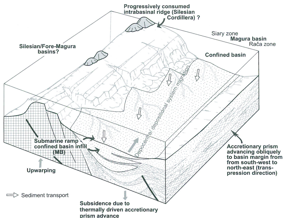
Fig. 30. Model of depositional system and sedimentation evolution of the Magura Beds during Priabonian–Rupelian
