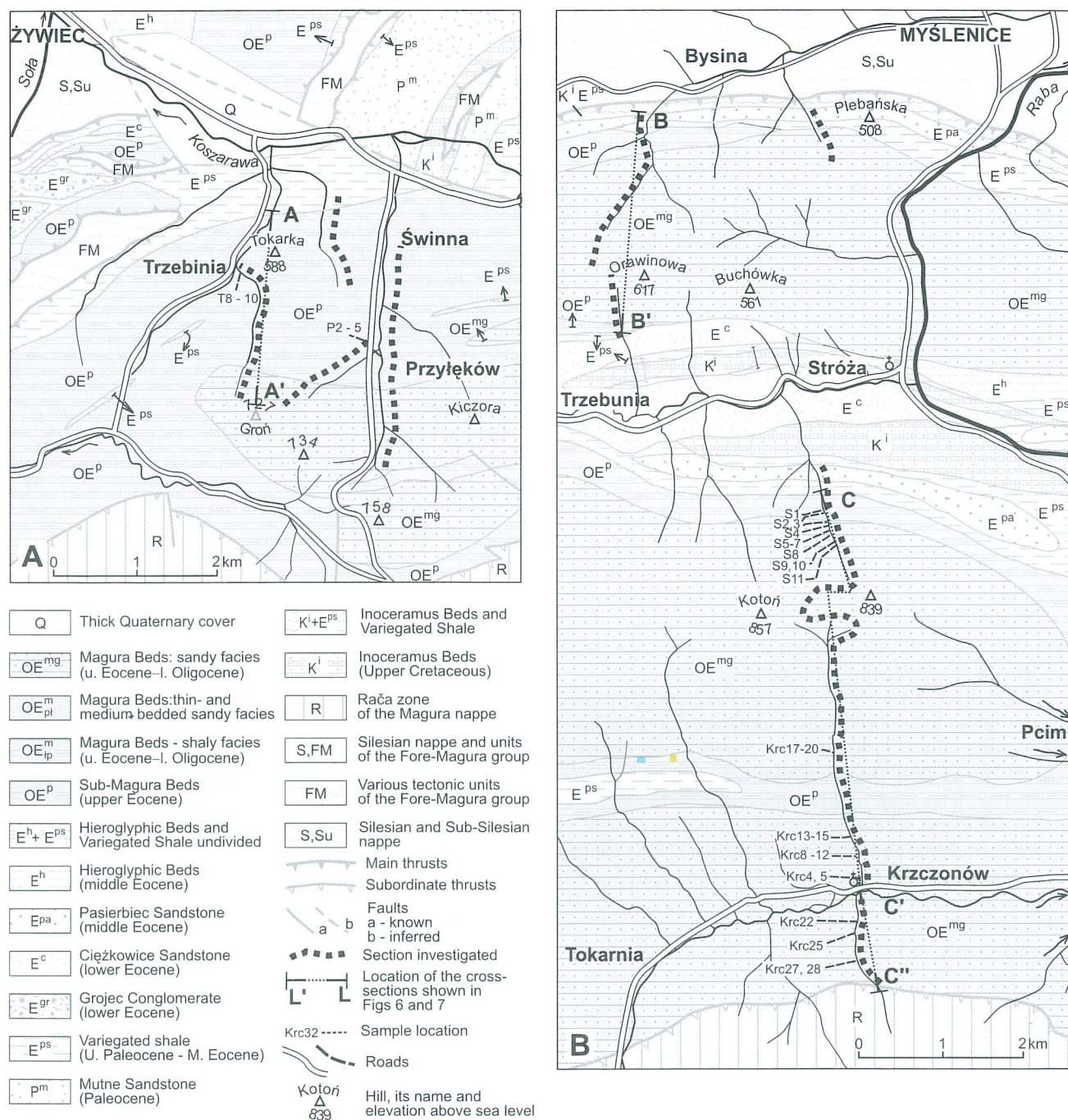
Fig. 3. Location of the sections measured in the western part of the Siary zone; location of samples mentioned in the paper and lines of cross-sections illustrated in Fig. 6. Geology of the area in A – according to Nowak (1966a, b), Sikora (1966) and Żytko (1966), in B – according to Burtan & Szymakowska (1966), slightly modified by S. Leszczyński. Note differences in stratigraphy of the sections indicated by these maps and author's data shown in Fig. 6
