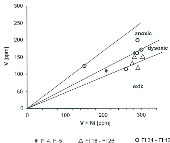
Fig. 29. Vanadium/vanadium + nickel plot of the fine grained-sediments from the Szymbark Shale (samples FI4, 5 – lower part; samples FI16-FI26 – upper part) and the lower part of Magura Beds (samples FI34-FI42) in the Folusz section. The fields of oxygenation regime are after Lewan (1984)
