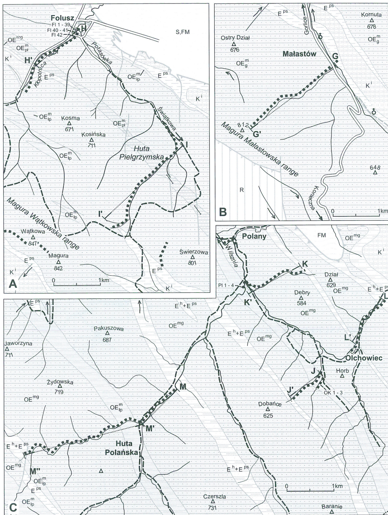
Fig. 5. Location of the sections measured in the eastern part of the Siary zone; location of samples mentioned in the paper and lines of cross-sections illustrated in Fig. 7. Geology of the area in A – according to Koszarski & Tokarski (1967), in B – according to Sikora (1967), in C – according to Ślącza (1967), slightly modified by S. Leszczyński. Note differences in stratigraphy of the sections indicated by the maps and author's data shown in Fig. 7. Symbols and abbreviations as in Fig. 3
