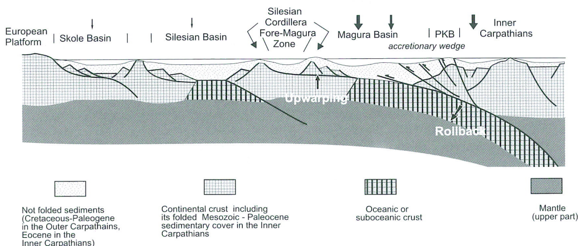
Fig. 31. Simplified palinspastic cross-section through the Northern Carpathians at the turn of the Eocene/Oligocene. Not to scale. Arrows denote relative subsidence rate
