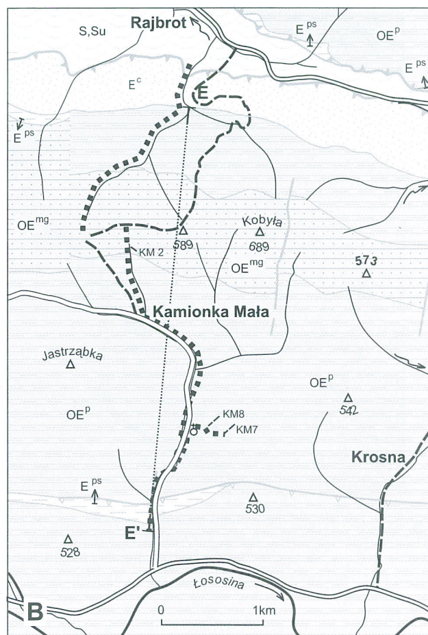
Fig. 4. Location of the sections measured in the central part of the Siary zone; location of samples mentioned in the paper and lines of cross-sections illustrated in Fig. 6. Geology of the area in A – according to Burtan (1966), in B – according to Burtan & Skoczylas-Ciszewska (1966a, b) and Cieszkowski (1992), slightly modified by S. Leszczyński. The sandstone unit marked E^c was named Ciężkowice Sandstone by Burtan & Skoczylas-Ciszewska (1966a, b) whereas Cieszkowski (1992) distinguished it as Wojakowa Sandstone. Note differences in stratigraphy of the sections indicated by these maps and author's data shown in Fig. 6. Symbols and abbreviations as in Fig. 3
