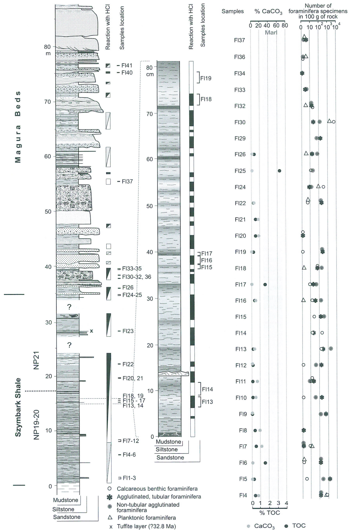
Fig. 26. Graphic log of the Szymbark Shale and the lower part of Magura Beds outcropped in the bed of Kłopotnica stream in Folsz (see Fig. 5A for section location), reaction with diluted HCl, TOC, CaCO 3 and foraminifera contents in the fine-grained sediments. Calcareous nannoplankton zones cf. Tab. 1 and Oszczytko-Clowes (2000, 2001). For other symbols, see Fig. 9
