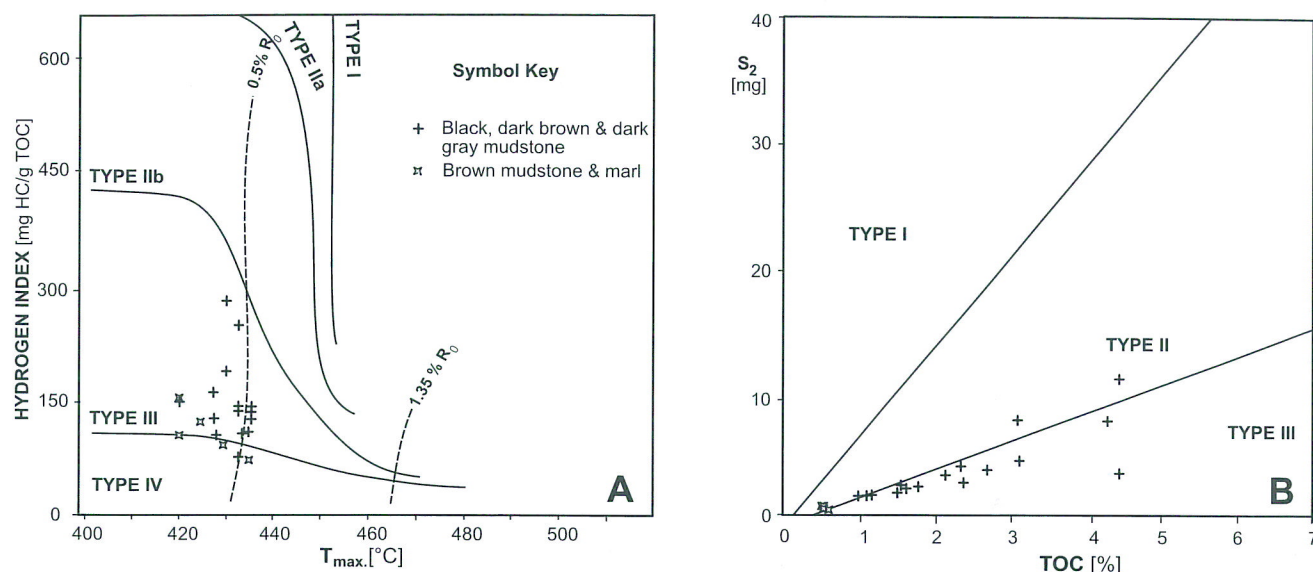
Fig. 28. Type of kerogen determined by Rock-Eval pyrolysis in the fine-grained rocks in which TOC exceeds 0.5%. A. Type of kerogen indicated by the relation between hydrogen index and the temperature of maximum hydrocarbon evolution ( T_{max} ). B. Type of kerogen indicated by the relation between total organic carbon content (TOC, in %) and the amount of hydrocarbons evolved from the thermal alteration of the kerogen ( S_2 in milligrams, normalized to sample weight)
