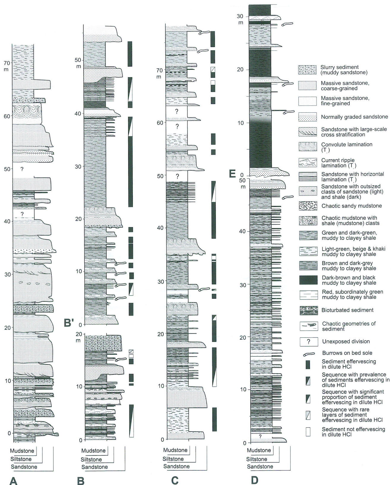
Fig. 9. Characteristic facies patterns (cf. general facies types in Figs. 7 and 8) and reaction of fine-grained sediments with diluted HCl in the Magura Beds. Sediment structures of siltstones and sandstones are shown in thick beds only. Thin and medium sandstone and siltstone beds (shown as lines) display structures of the divisions T_{(ab)c} and T_{(c)d} of the Bouma sequence respectively. Logs A–D represent succession segments shown in Fig. 8. Log E shows section of the upper part of Magura Beds in the bed of Wistoka river between villages Czarne and Nieznajowa (between areas E and G in Fig. 1). Note vertical variation of carbonate content in fine-grained sediments
