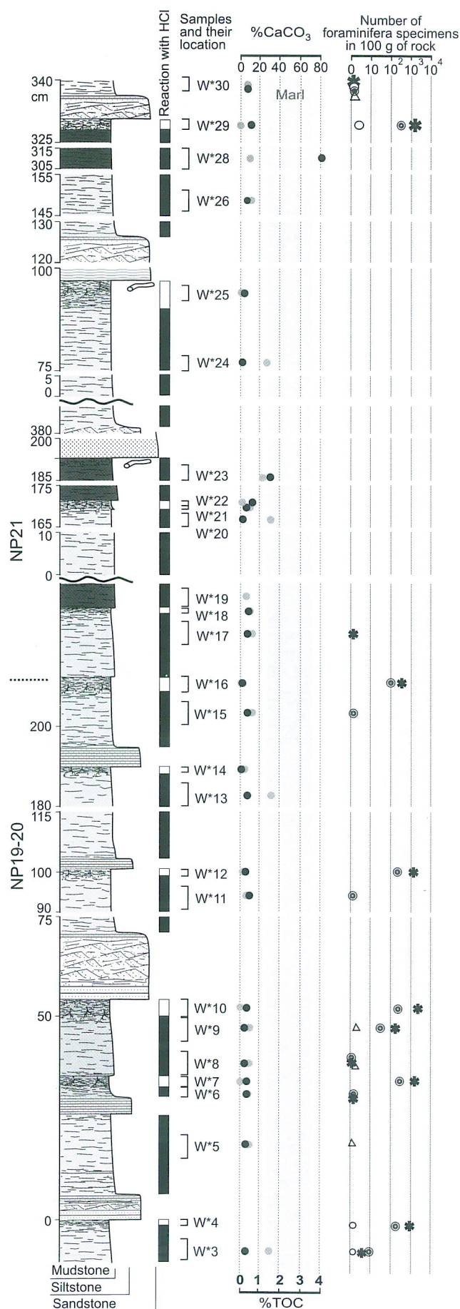
Fig. 27. Graphic log of the sampled lower part of Magura Beds outcropped along the road between Kobielnik and Węglówka villages (see Fig. 4A for section location), reaction with diluted HCl, TOC, CaCO 3 and foraminifera contents in the fine-grained sediments. Calcareous nannoplankton zones cf. Tab. 1. For other symbols, see Fig. 9
