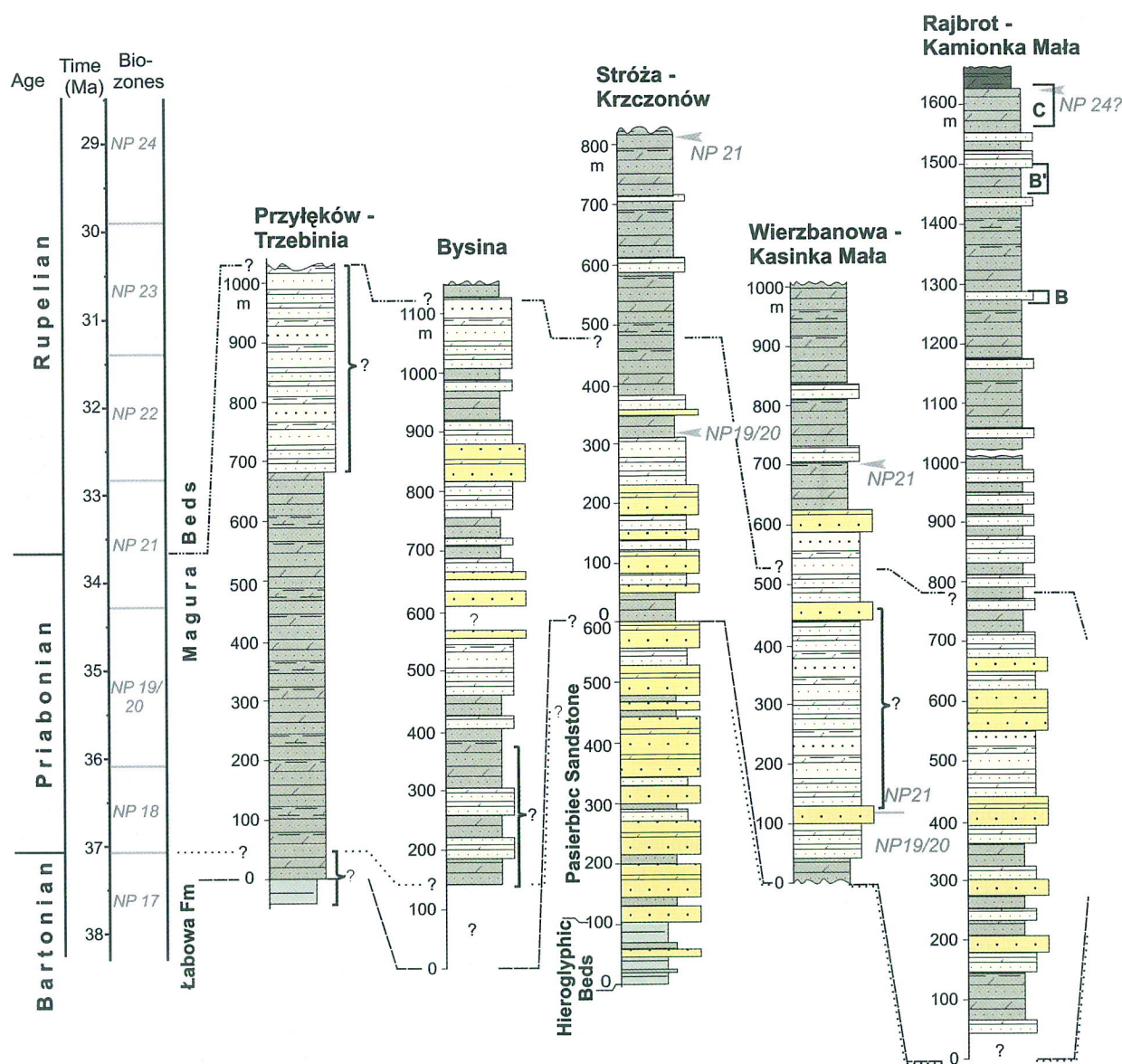
Fig. 8. Generalised logs of the Priabonian–Rupelian of the Siary zone and their correlation (see Figs 3–5 for sections location). Facies as these shown in Fig. 6. Chronostratigraphy based on Sikora & Żytka (1960), Blaicher & Sikora (1963), Sikora (1970), Malata (1981, 2001), Jednorowska (1966), biostratigraphy based on Oszczypko-Clowes (1999, 2000, 2001) and datations done by Oszczypko-Clowes in the frame of this project (see Tab. 1). Biozones according to Martini (1971) correlated with chronostratigraphic and time scales by Berggren et al. (1995). Note that the Magura Beds in the logs from the western part of the Siary zone are basically of Priabonian age whereas these from the eastern part are mainly Rupelian. The top of this unit is erosional and seems to not stride lower Rupelian in the western part of the Siary zone, while in the east it reaches the top of Rupelian
