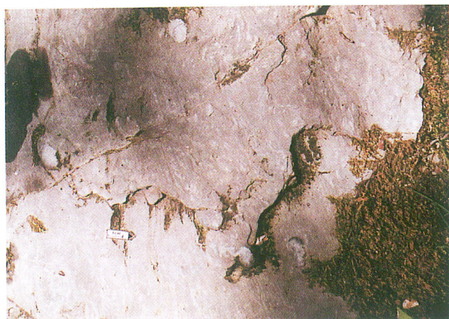
Fig. 23. Chaotic sandy mudstone with rounded clasts of sandstone (balled mudstone). Scale 17 mm long in the lower centre. Upper part of Magura Beds (Budzów Shale), Krzczonów
