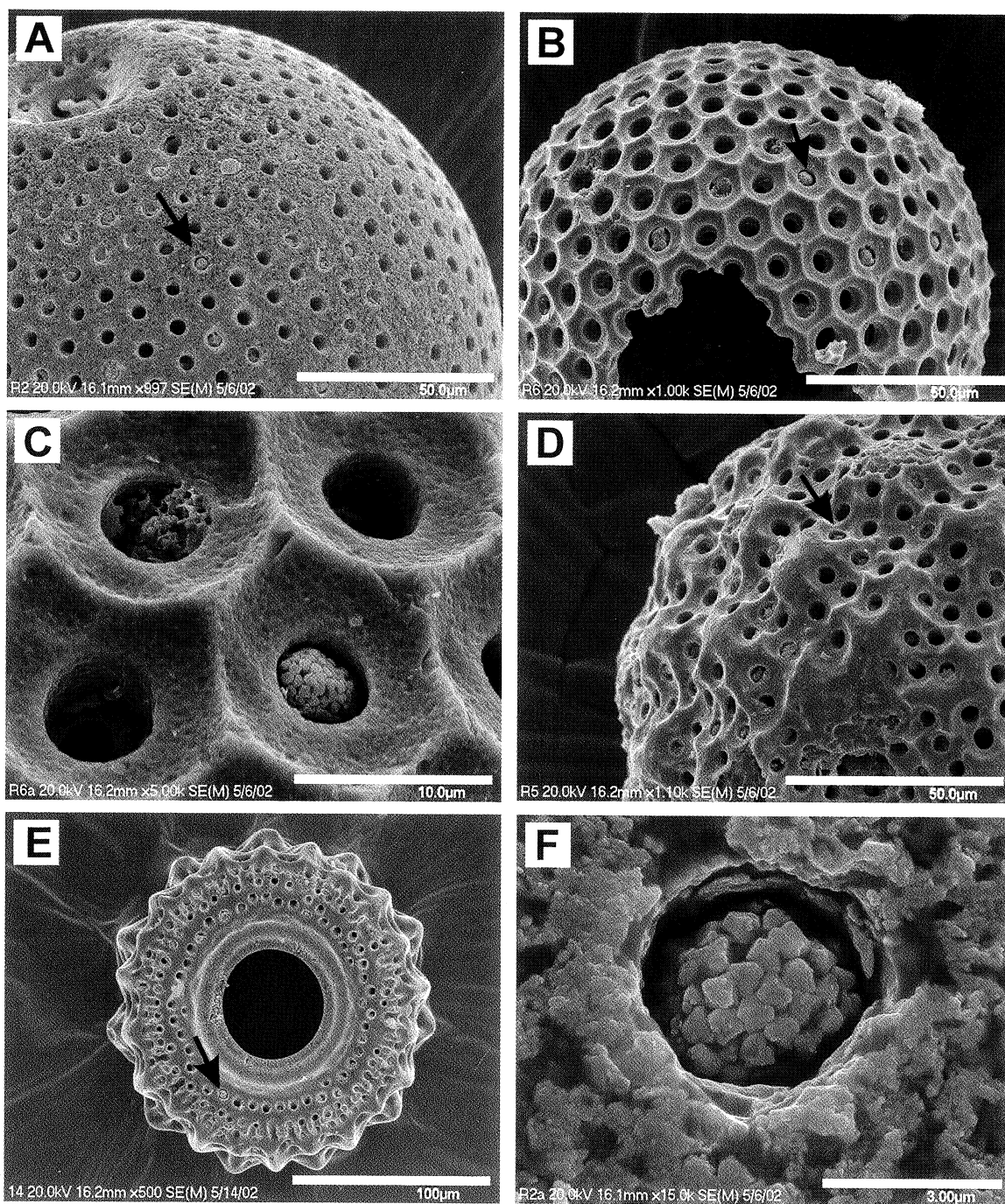
Fig. 1. Examples of framboids from pyritized radiolaria. A – pyritized radiolarian skeleton ( Holocryptocanium barbui Dumitrica) with pyrite framboids visible in the uppermost parts of pores (scale bar 50 µm); B – pyrite framboids visible in lower parts of pores (arrow, compare with Fig. 1A) of the uncovered by erosion outermost layer of pyritized radiolarian skeleton of H. barbui (scale bar 50 µm); C – pyrite framboid and irregular cluster of pyrite crystals in pores of pyritized H. barbui (magnified fragment of Fig. 1B; scale bar 10 µm); D – pyritized radiolarian skeleton ( Holocryptocanium tuberculatum ) with pyrite framboids visible in pores (scale bar 50 µm); E – pyrite framboids visible in the last chamber of pyritized Xitus mclaughilini Pessagno (scale bar 100 µm); F – pyrite framboid with intergrown microcrystals in a pore of pyritized skeleton of H. barbui (scale bar 3 µm)
