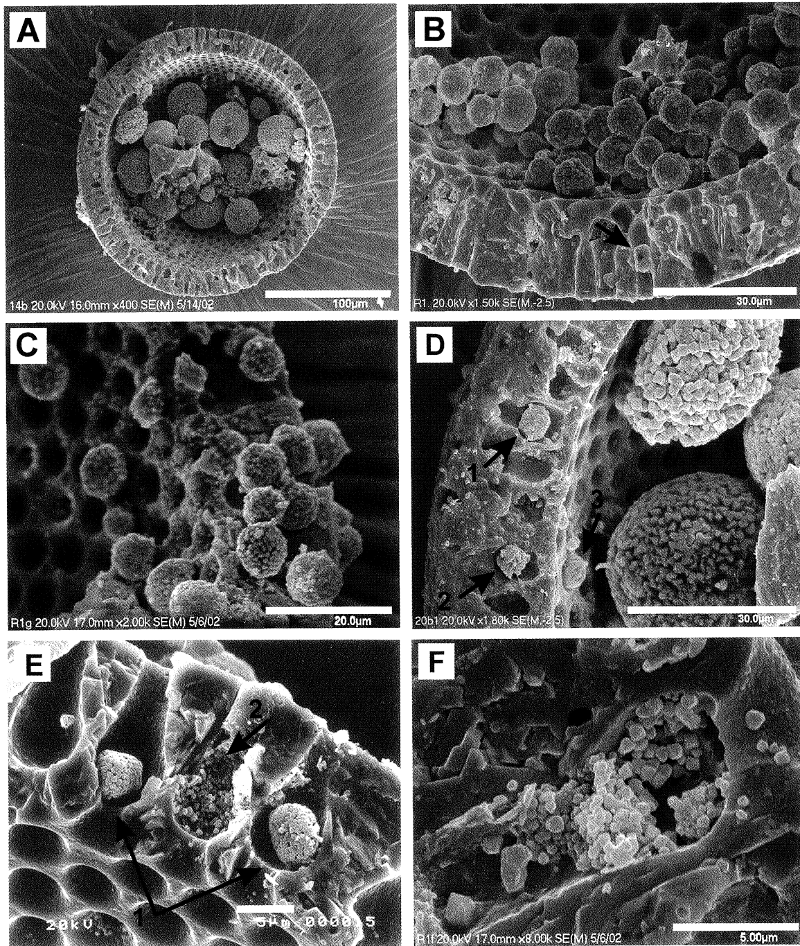
Fig. 2. Examples of framboids from pyritized radiolaria. A – cross-section of pyritized H. barbui : cluster of pyrite framboids of various sizes in the interior of the abdominal chamber (scale bar 100 \mu\text{m} ); B – cross-section of pyritized H. barbui : cluster of pyrite framboids of uniform sizes in the interior of the abdominal chamber (some of the framboids are attached to channels exits; arrowed framboid modified by the shape of channel; scale bar 30 \mu\text{m} ); C – pyrite framboids attached to inner, outer and broken parts of pyritized H. barbui (growth on the broken skeleton in a sediment or artificial destruction during laboratory preparation?; scale bar 20 \mu\text{m} ); D – cross-section of pyritized H. barbui : angular “hipidiomorphic” (1) and irregular in outline (2) pyrite framboids in pores; (3) – pyrite framboid attached to a channel exit (scale bar 30 \mu\text{m} ); E – crystal-like pyrite framboids in the so-called lamp chimney-like pores of H. barbui : (1) – the shapes are probably modified by the shape of pores (framboids removed from their primary position?); (2) – a pore filled by the aggregate of pyrite micro-crystals (scale bar 5 \mu\text{m} ); F – framboidal aggregate (disintegrated framboid or encrustation of channel inner surface?) inside of a channel of H. barbui (scale bar 5 \mu\text{m} )
