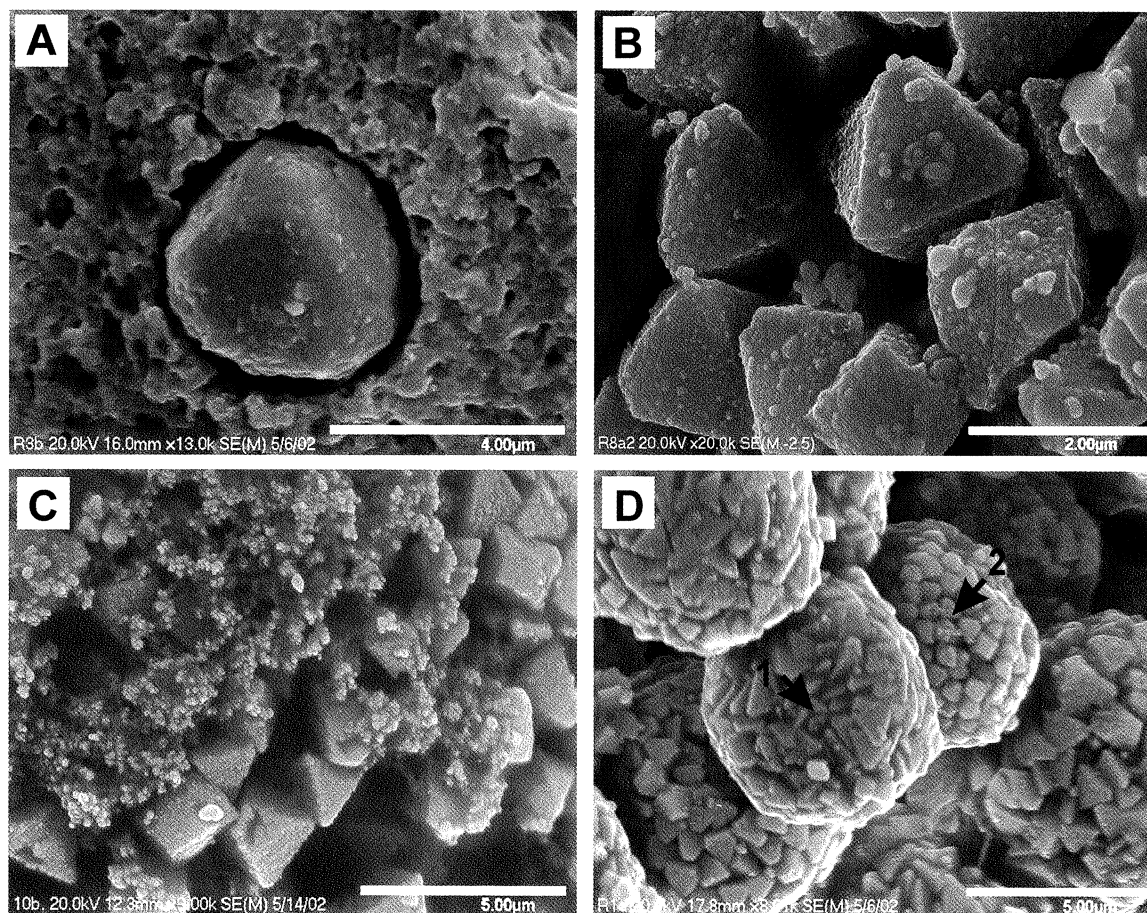
Fig. 3. Examples of pyrite from pyritized radiolaria. A – pyrite euhedra (possibly recrystallized framboid) in a pore of pyritized H. barbui (scale bar 4 μm); B – octahedral microcrystals of pyrite framboid from the abdomen of pyritized H. barbui (note that microcrystals are built of smaller subunits ranging from 50 to 100 nm – crystal-like microframboid sensu Sawłowicz, 1993; scale bar 2 μm); C – pyrite octahedral microcrystals (see Fig. 3B) encrusted by minute (200–300 nm) pyrite grains (abdomen of pyritized H. barbui ; scale bar 5 μm); D – pyrite framboids built of closely packed (1) and strongly intergrown microcrystals (2) (pyritized H. barbui ; scale bar 5 μm)
