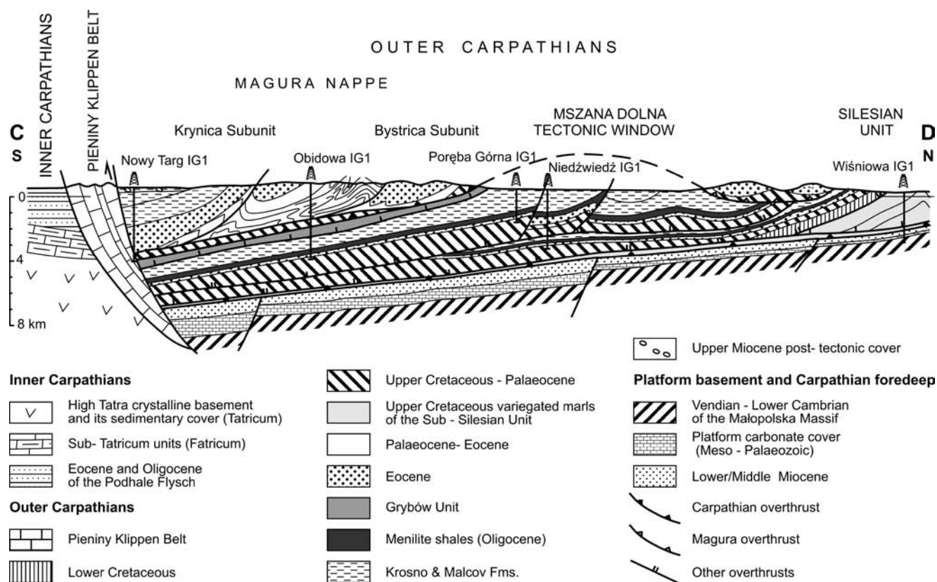
Fig. 4. Geological cross-section through the medial segment of the Magura Nappe (based on Oszczypko, 2006). For location see Fig. 1.
