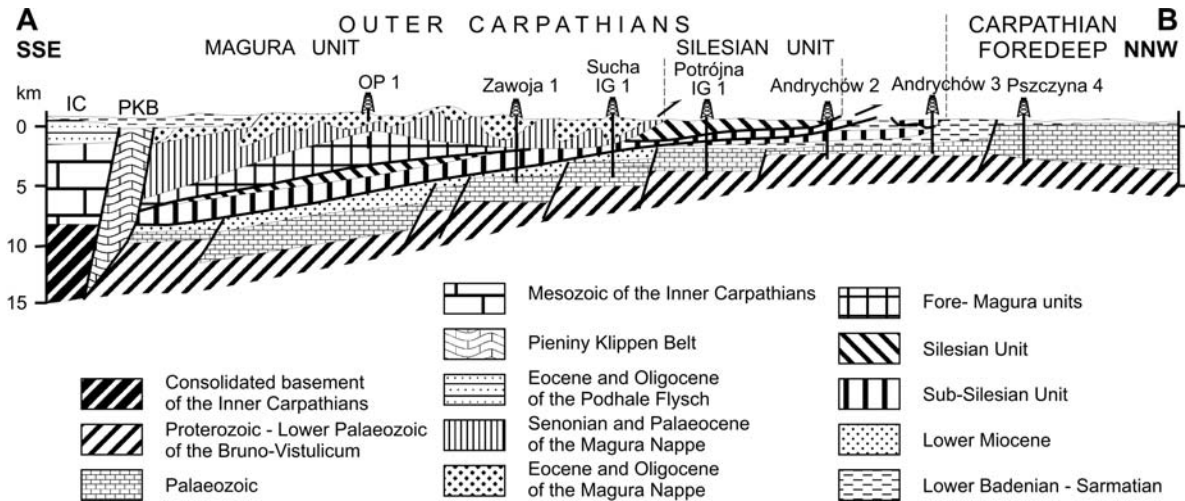
Fig. 3. Geological cross-section through the western portion of the Magura Nappe (based on Oszczypko et al. , 2006). For location see Fig. 1. IC – Inner Carpathians, PKB – Pieniny Klippen Belt, OP 1 – Oravska Polhora 1 borehole
