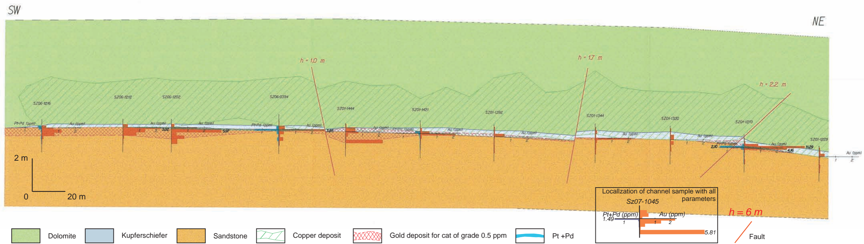
Fig. 81. Cross section P2u along mining work K-4, Polkowice Mine, East Field
