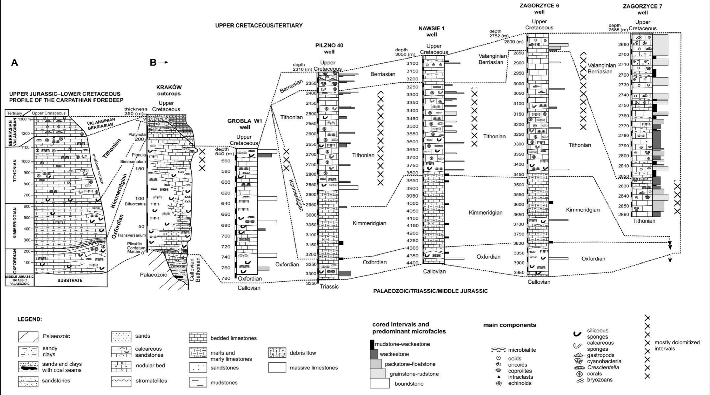
Fig. 3. A – a general lithological section of the southern part of the Upper Jurassic–Lower Cretaceous Carpathian Foredeep basement deposits between Kraków and Rzeszów; in the western part (Kraków area) only Oxfordian–Lower Kimmeridgian sediments were found; Tithonian, Berriasian and Valanginian sequence is representative for the Tarnów–Ropczyce area only, B – lithological logs of the main studied well sections and outcrops from the Kraków–Rzeszów area
